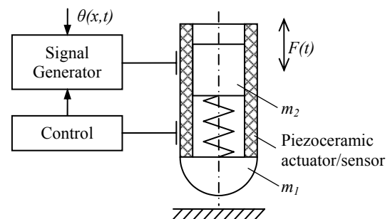
Fig. 1. Controlling the structure of impact system
