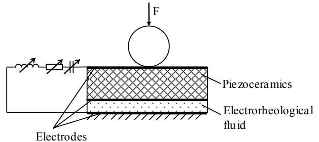
Fig. 6. Composite structure of active materials
