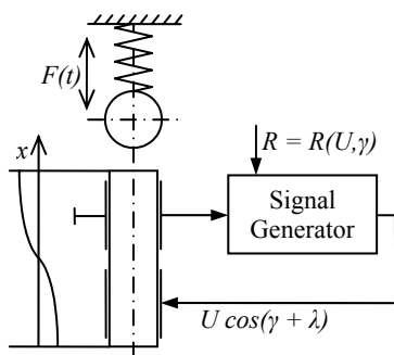
Fig. 5. Coefficient of restitution control, using piezoceramics
