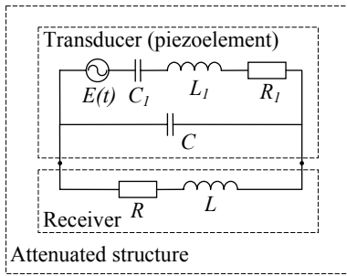
Fig. 3. Equivalent circuit of the tested system
