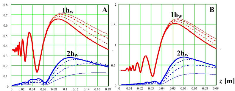
Fig. 2. The 1-st (top 4 lines) and the 2-nd (bottom 4 lines) harmonic axial distributions for the case of 8-cycle pulse with the carrier frequency of 2 MHz, radiated by the plane (left) and focused (right) source of 10 mm radius, when the initial acoustic pressure amplitude p_0 is equal to 0.1 (thin solid lines); 0.2 (dashed lines); 0.3 (dotted lines); 0.4 (thick solid lines) MPa
