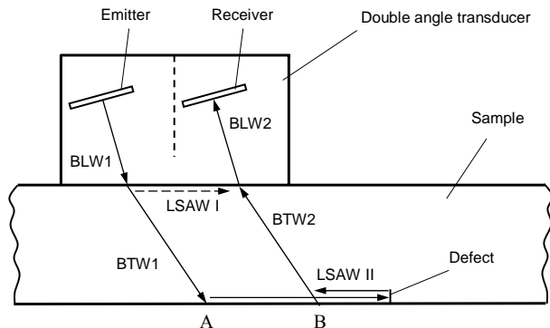
Fig. 6. Double angle transducer
