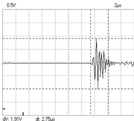
Fig.7. LSAW II signal received by the angle transducer (1) at 2.5MHz, propagating in the forward direction
