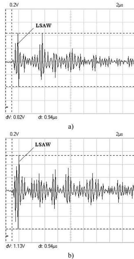
Fig.11. LSAW II signals, reflected from notch in plate with thickness D=10 mm. Depth of notch (defect) h : a - 2 mm; b - 4 mm.
