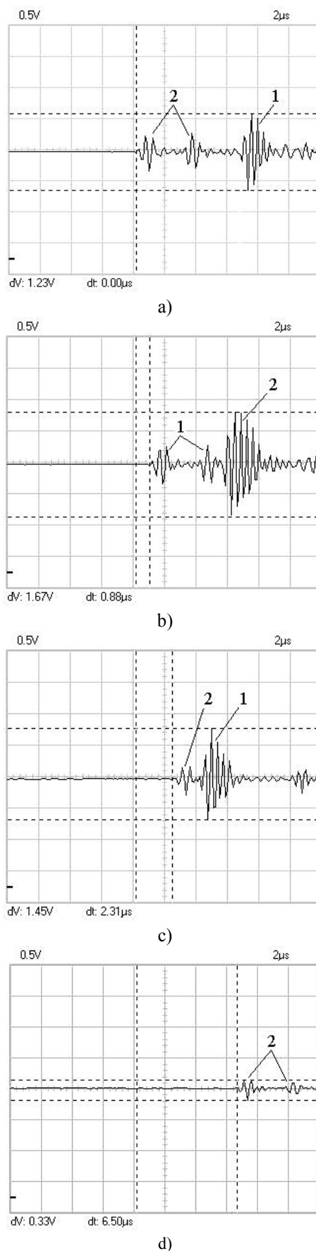
Fig.8. LSAW II signals (1), reflected from the sample notch ( h=2 mm); signals (2) received at the reverse direction of transducer. Distance L from pick-up aperture center to defect: a) +4 mm; b) 0 mm; c) -19 mm; d) -48 mm
