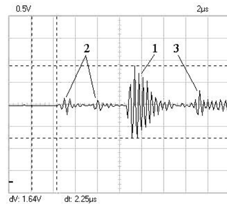
Fig. 5. LSAW signal on the display of a digital oscilloscope: 1 – LSAW, pulse, reflected from the defect; 2 – duplicated collateral (forward) LSAW pulses, picked by the receiver in the reverse direction; 3 – repeated piezoelement excitation pulse, reflected from the defect
