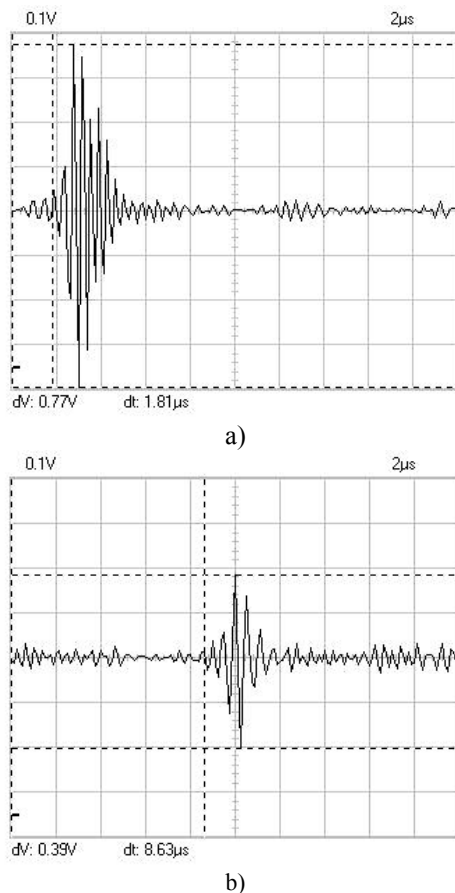
Fig.10. LSAW II signal, reflected from the inner defect, when D = 40 mm and the distance L : a - 0 mm; b - 20 mm
