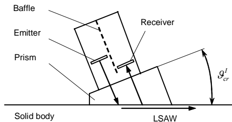
Fig. 4. LSAW angle transducer with additional prism
