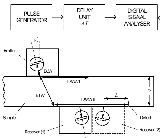
Fig. 1. LSAW II experimental investigation scheme
