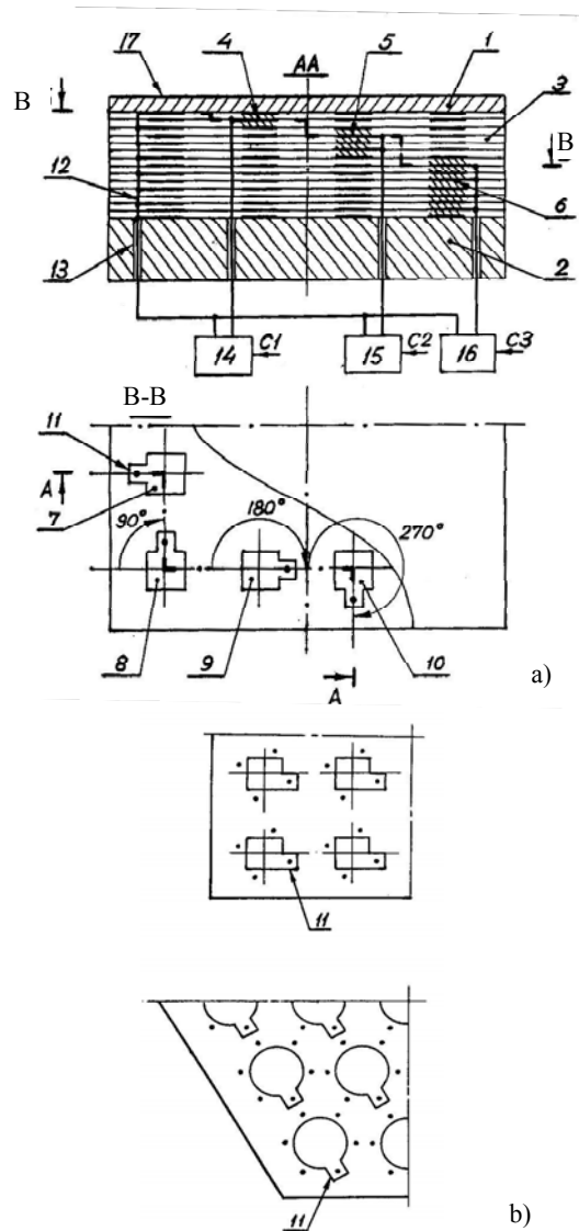
Fig.3. Wave-front phase modulator: 1 – mirror; 2 – rigid base; 3 – multilayer unit; 4, 5, 6 – sections; 7, 8, 9, 10 – address electrodes; 11 – protuberances; 12 – conductors; 13 – holes; 14, 15, 16 – digital electronics switch
