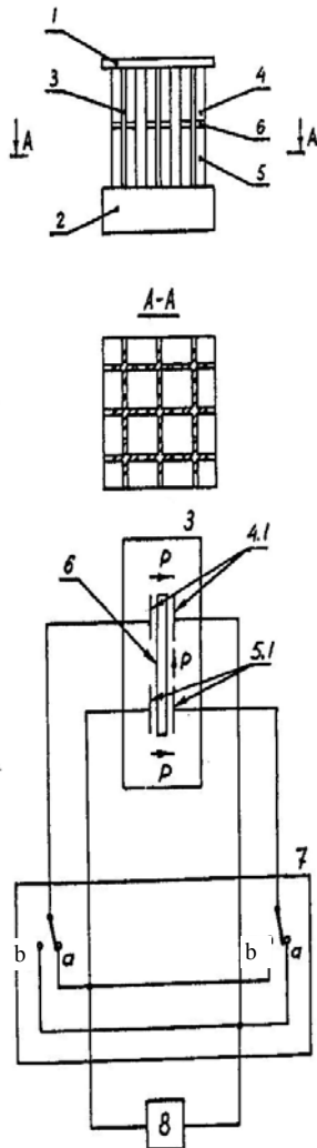
Fig.2. Construction phase modulator: 1 – mirror; 2 – rigid base; 3 – piezoelectric elements; 4, 5 – electrodes; 6 – gap; 7 – switch; 8 – control voltage
