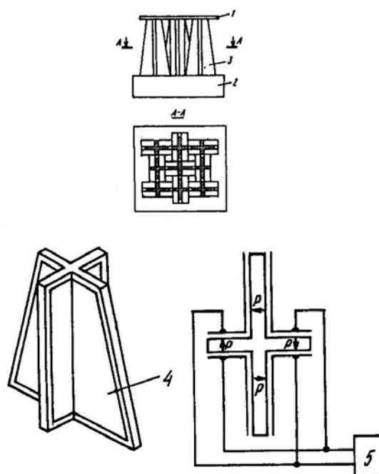
Fig.1. The construction and diagram of electric connections of the wave-front phase modulator: 1 – mirror; 2 – rigid base; 3 – piezoelectric elements; 4 – control electrodes; 5 – control voltage
