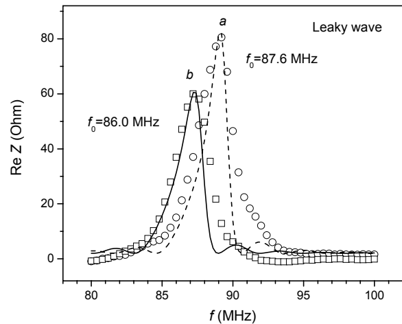
Fig. 7. Real part of IDT impedance for leaky waves. Sample S1. Dots, experiment. Lines, theory with fitting parameters: a) non-exchanged surface, V=4380 \text{ m/s} , K^2=3.1\% ; b) proton-exchanged surface, V=4300 \text{ m/s} , K^2=2.5\% . The center frequencies f_0 are indicated at the corresponding curves
