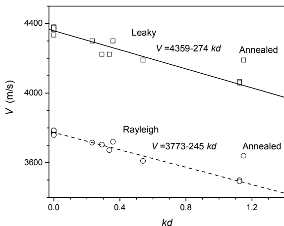
Fig. 9. Leaky and Rayleigh SAW velocities in proton-exchanged ZX LiNbO 3 as functions of wave number-layer thickness product kd . Dots, experiment; lines, linear approximations with slopes indicated. The V values obtained in a post-annealed sample are also shown
