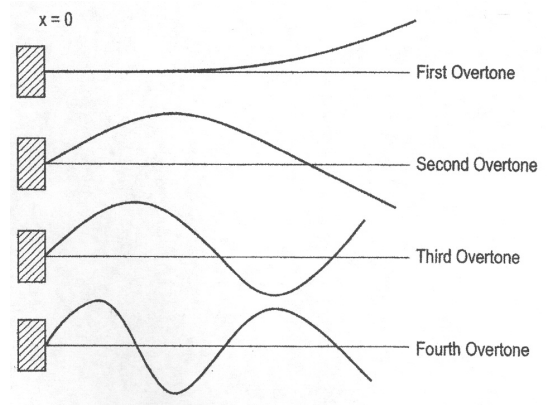
Fig.3. Transverse vibration modes.
