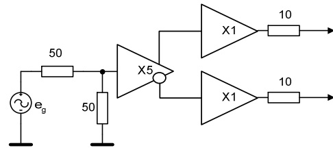
Fig. 4. Driving generator structure
