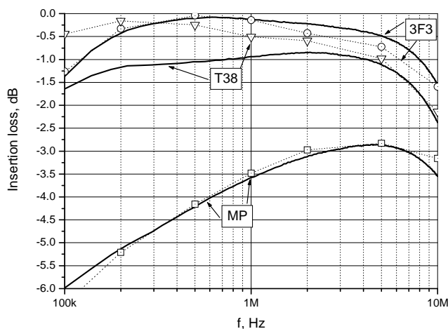
Fig. 5. Insertion loss measurement and modelling
