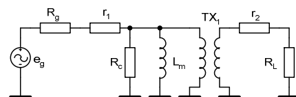
Fig. 2. Low frequency region equivalent circuit
