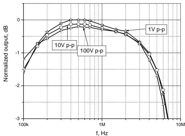
Fig. 6. Normalized output voltage frequency response
