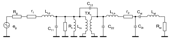
Fig. 1. Transformer coupled excitation equivalent circuit
