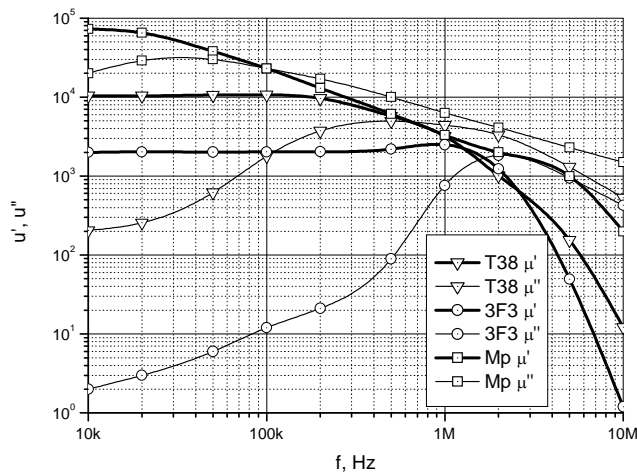
Fig. 3. Complex permeability of the candidate materials
