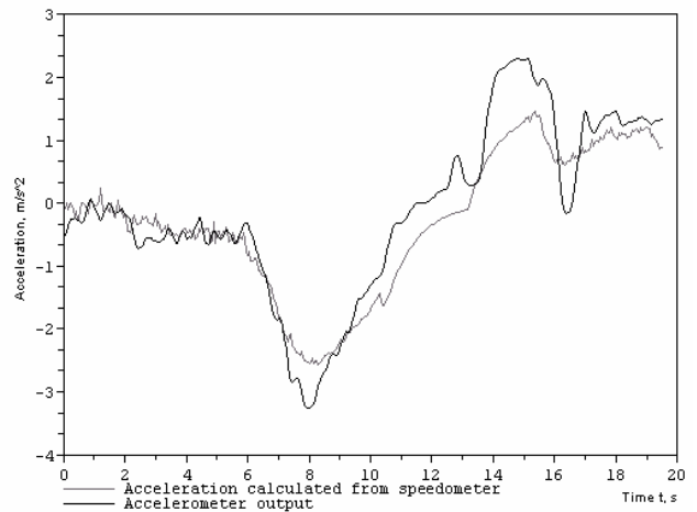
Fig. 10. Accelerometer output from x_s axis and acceleration calculated from speedometer signal. Data acquired on on-road test with use of Fiat Punto
