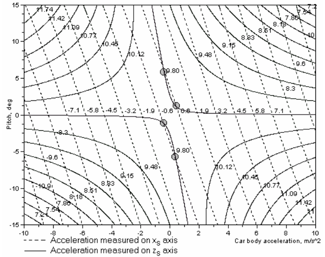
Fig. 9. Simulated acceleration measured on x_s and z_s axis and real car body acceleration as a function of car body acceleration and pitch angle
