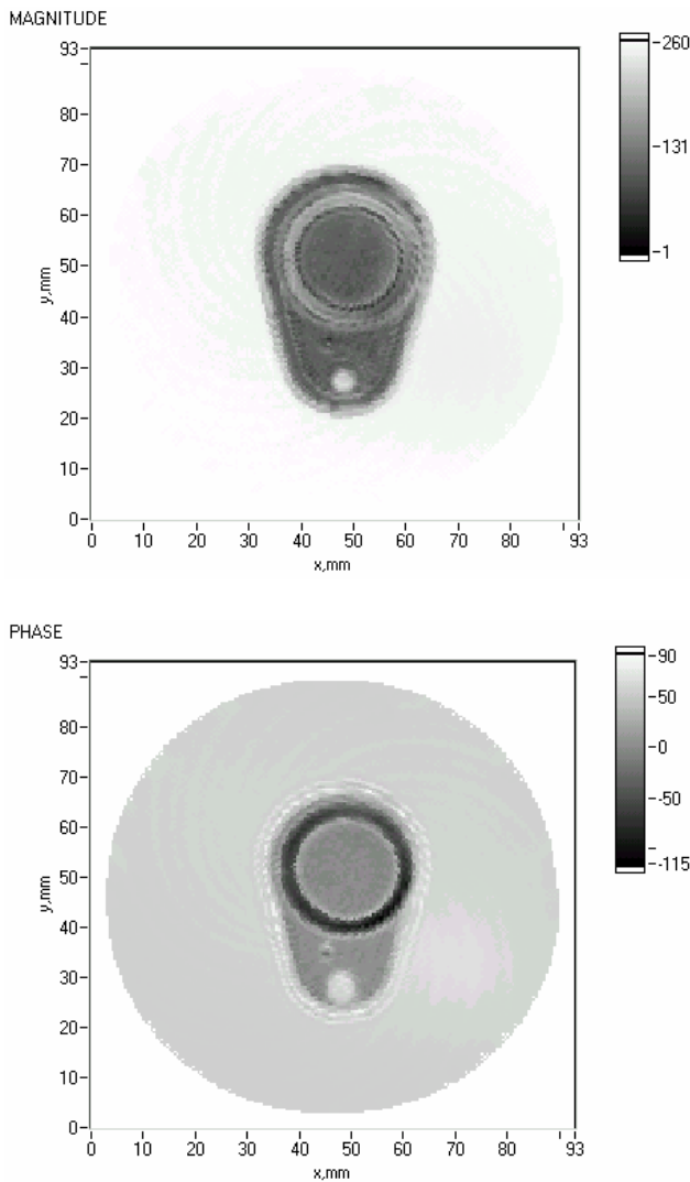
Fig. 4. Millimetre wave amplitude (top) and phase (bottom) images of the door electronic key transponder. Wave frequency is 120GHz.
