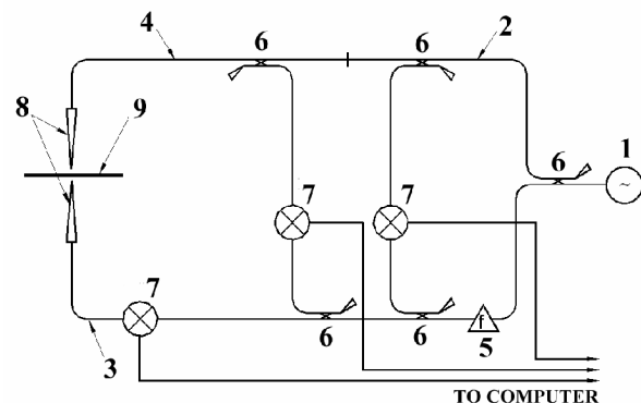
Fig. 1 Schematic diagram of the device measuring transmitted and reflected electromagnetic wave amplitude and phase: 1 is millimeter wave oscillator, 2 is reference signal channel, 3 is transmitted signal channel, 4 is reflected signal channel, 5 is frequency converter, 6 are directional couplers, 7 are mixers, 8 are antennas, and 9 is the sample under test.
