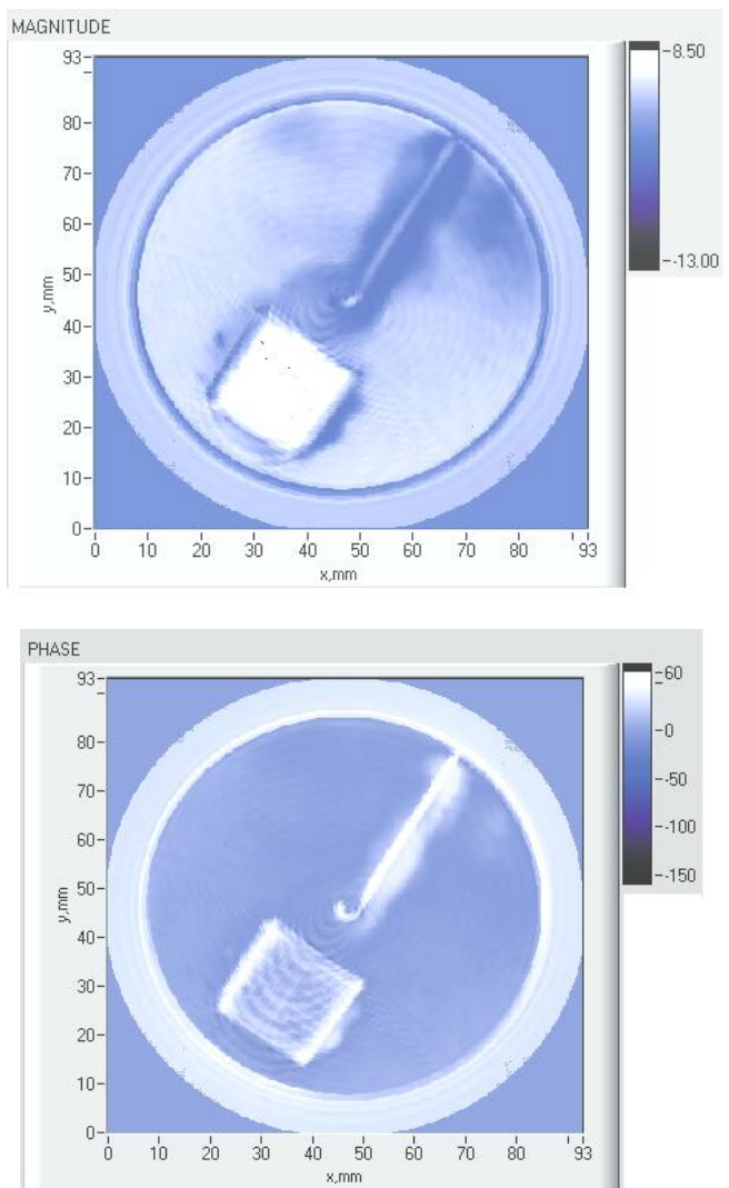
Fig. 5. Millimetre wave amplitude (top) and phase (bottom) images of the metallic plate with local destructive surface under paint. Wave frequency is 120 GHz.
