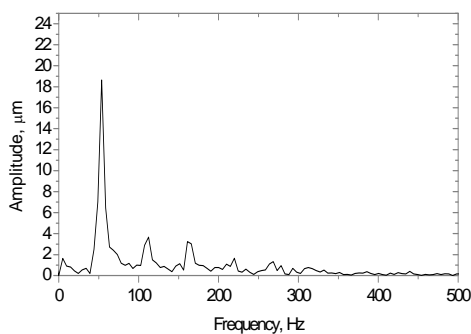
Fig. 5. Spectrum of signals that are obtained measuring rotary system with sliding bearings, clearance is 100 \mu\text{m} rate of rotor revolution 3000 rev/min
