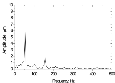
Fig. 4. Spectrum of signals that are obtained measuring rotary system with bearings of sliding, clearance is 50 μm, frequency of rotor revolution 3000 rev/min
