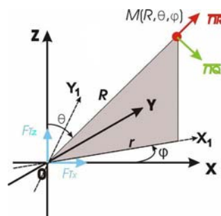
Fig. 1. Calculation scheme for field of normal F_z or tangential F_x harmonic force source
