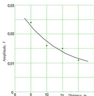
Fig. 13 Echo-signal amplitude from the rail's butt-end versus the distance between the antenna array and the butt-end
