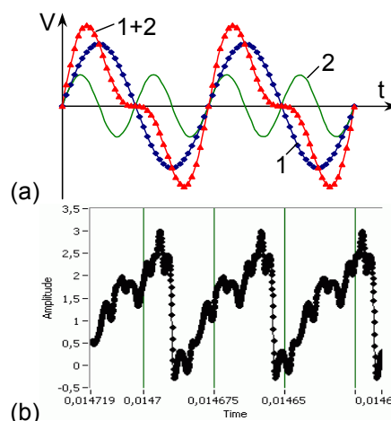
Fig.2. Approximation of saw-tooth oscillations comprised of two harmonics (a); experimental response of the actuator driven by a single saw-tooth signal (b)
