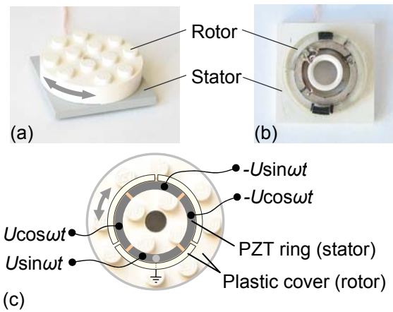
Fig.5. Prototype (a) and schematic (b, c) of the rotational "smart" brick
