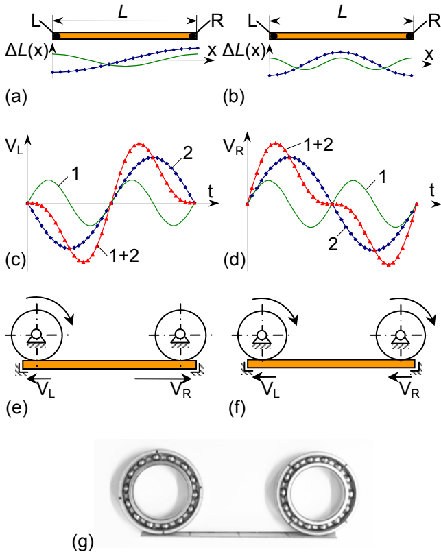
Fig.3. Actuator's strains (a), speeds (c,d) and synchronization (e) with the first and the second longitudinal modes superimposed; strains (b), speeds (c) (same for "L" and "R") and synchronization (f) with the second and the fourth longitudinal modes superimposed; motor's prototype (g)
