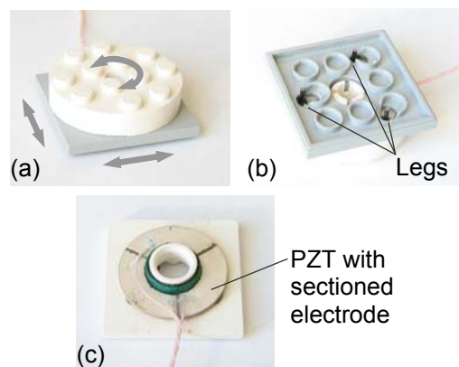
Fig.6. Top (a), bottom (b) and setup (c) views of the three degree-of-freedom "smart" brick
