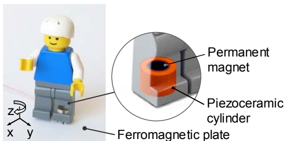
Fig. 4. Prototype of the "smart" minifigure
