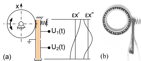
Fig. 1. Inertial piezomotor's schematics (a) and prototype (b)
