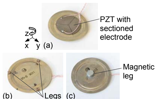
Fig.7. Top (a) and bottom (b-c) views of the three degree-of-freedom simplified motor
