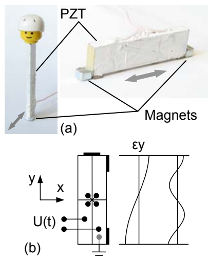
Fig.8. Prototypes (a) and schematics (b) of the linear piezoelectric motor
