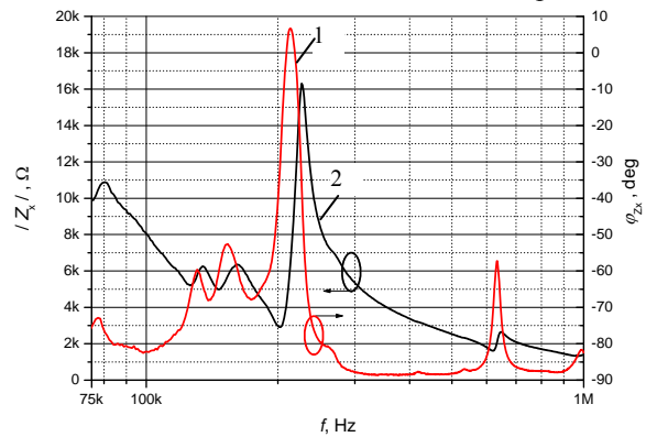
Fig. 3. Air coupled 200 kHz transducer impedance |Z_x| (1) and the phase \varphi_{z_x} (2) vs. frequency
