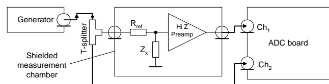
Fig. 1. Measurement setup
