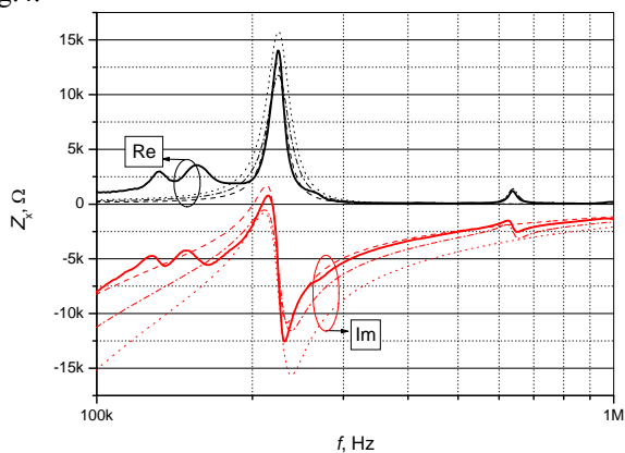
Fig. 4. Measured impedance approximation using the BVD model
