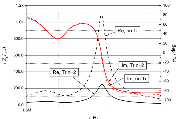
Fig. 7 Impedance modification by matching transformer
