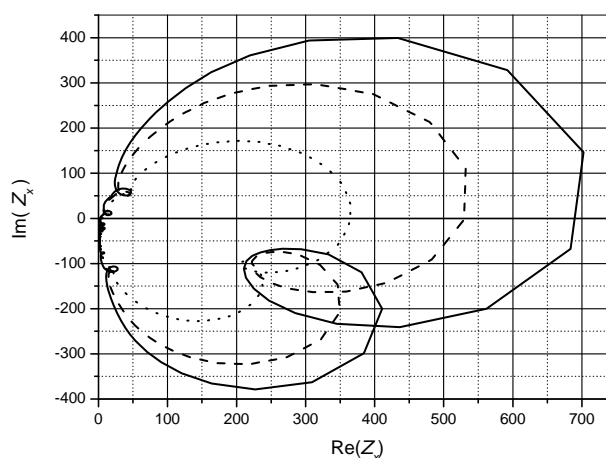
Fig. 5. Transducer Z_x polar plot in a complex coordinate system
