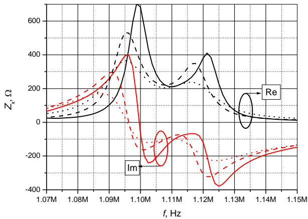
Fig. 6. PZT disk impedance variation with damping
