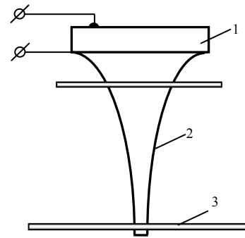
Fig.11. Cross section of composite transducer with transformation of vibrations: 1 – rectangular or circular piezotransducer; 2 – concentrator of acoustic waves; 3 – thin-walled rectangular elastic plate
