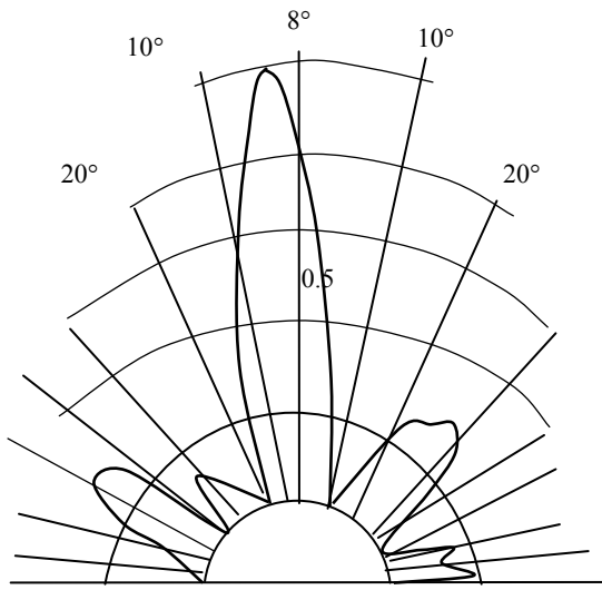
Fig.5. Directivity pattern of acoustic antenna (Fig. 4)
