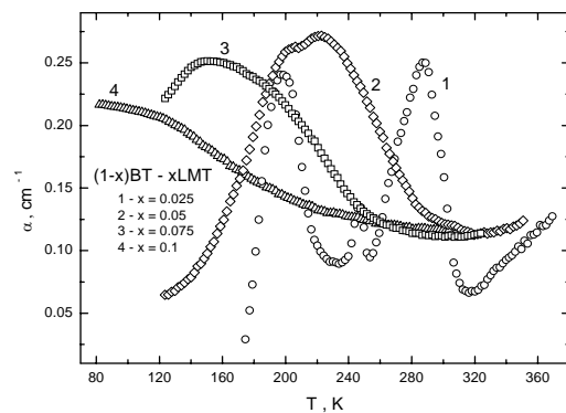
Fig.5 The temperature dependencies of longitudinal ultrasonic attenuation measured in unpolarised BT-LMT ceramics at 10 MHz frequencies
