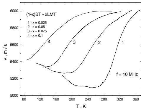
Fig.4. The temperature dependencies of longitudinal ultrasonic velocity measured in unpolarised BT-LMT ceramics at 10 MHz frequencies
