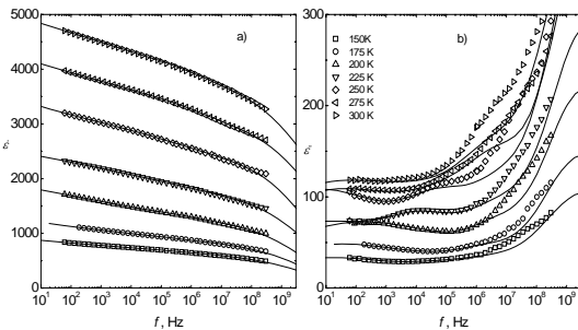
Fig. 2. Frequency dependences of the real (a) and imaginary (b) parts of the dielectric permittivity measured in different temperatures. Lines are the best fits with the obtained distribution of the relaxation times for BT-0.025LMT
