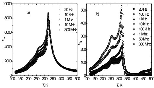
Fig. 1. Temperature dependence of the real (a) and imaginary (b) parts of dielectric permittivity at different frequencies of BT-0.025LMT
