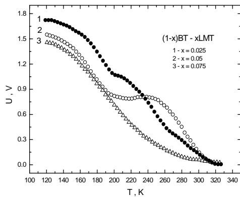
Fig.6. The temperature dependence of electric signal detected by BT_LMT ceramic plates
