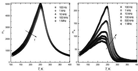
Fig.3. The temperature dependence of the real (a) and imaginary (b) parts of dielectric permittivity at different frequencies of BT-0.05LMT
