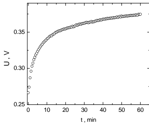
Fig.8. The time dependence of ultrasonic signal detected by BT-LMT plate. The applied DC field was 20 kV/cm.
