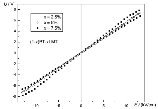
Fig.7. Dependencies of electric signal detected by BT-LMT plates with different composition on DC bias electric field
