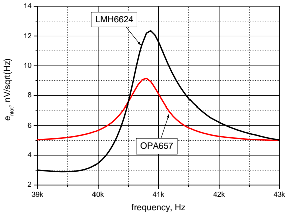
Fig. 4. Measured Prowave 400EP18D transducer voltage noise density
