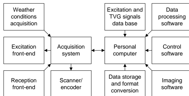
Fig. 1. Research system functional diagram
