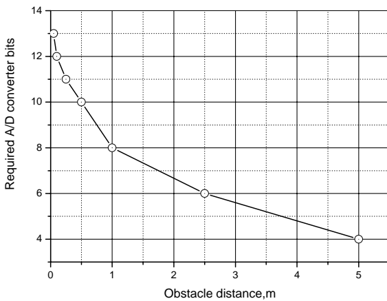
Fig. 5. Required A/D converter bits versus obstacle distance at 40kHz
