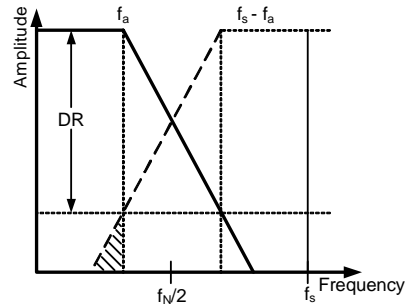
Fig. 6. Anti-aliasing filter requirements
