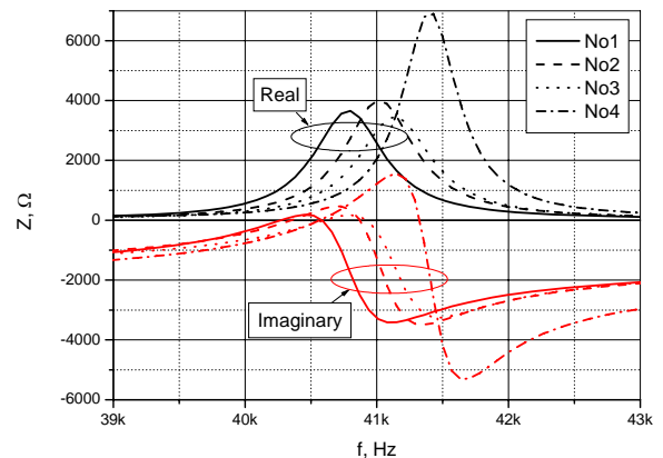
Fig. 3. Measured complex impedance of the Prowave 400EP18D transducer
