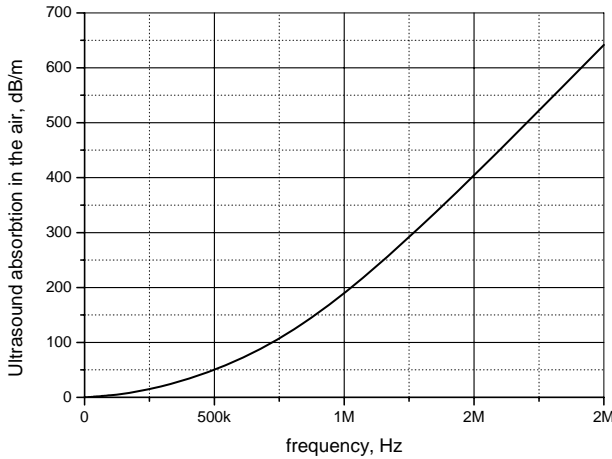
Fig. 2. Ultrasound absorption in air at 20°C 101kPa 60%RH
