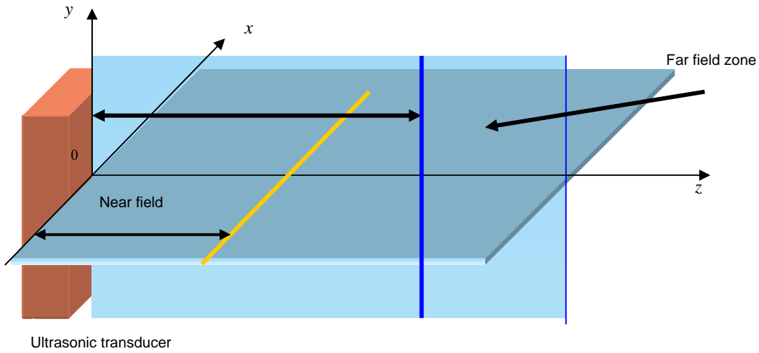
Fig. 4. Ultrasonic field of rectangular transducer in x0z and y0z planes
