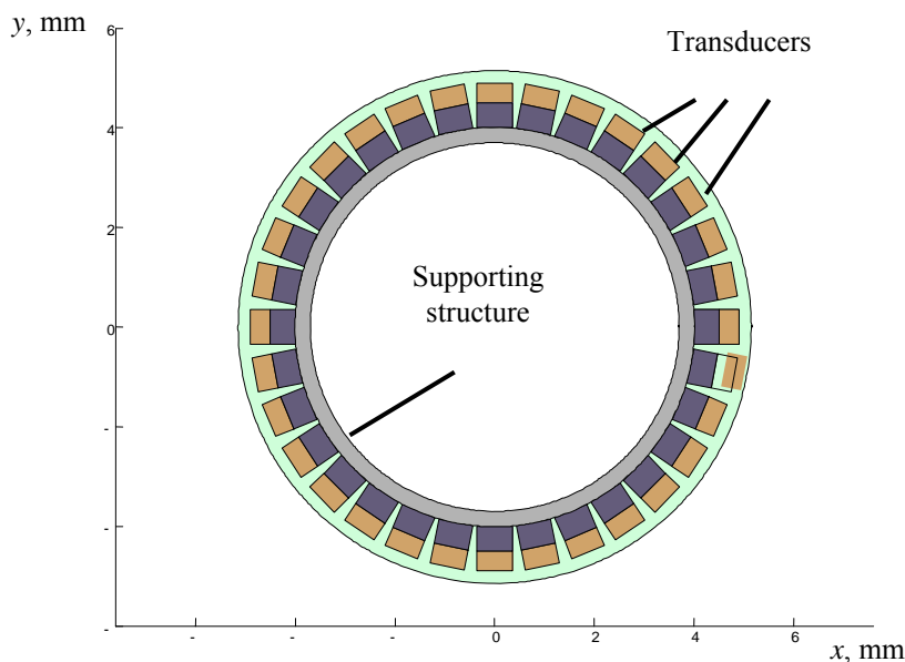
Fig.1 Ultrasonic array consisting of 32 separate transducers
