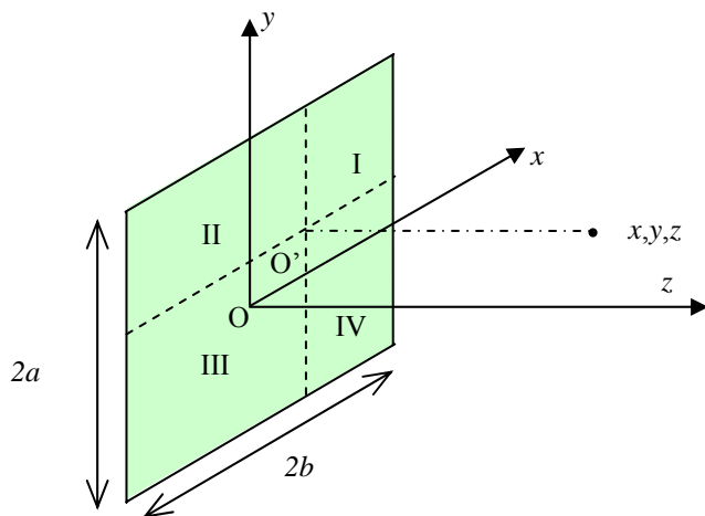
Fig. 3. Subdivision of the rectangular transducer into four rectangles
