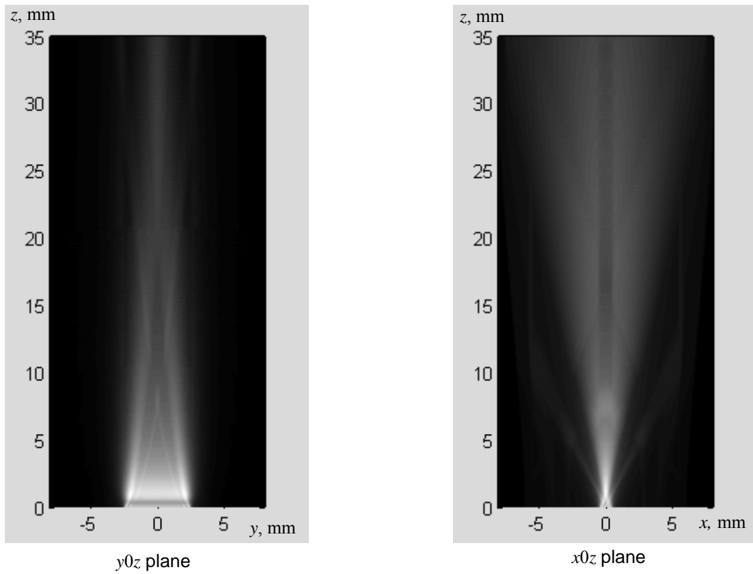
Fig. 6. Ultrasonic field of 5MHz transducer with dimensions 1x5 mm
