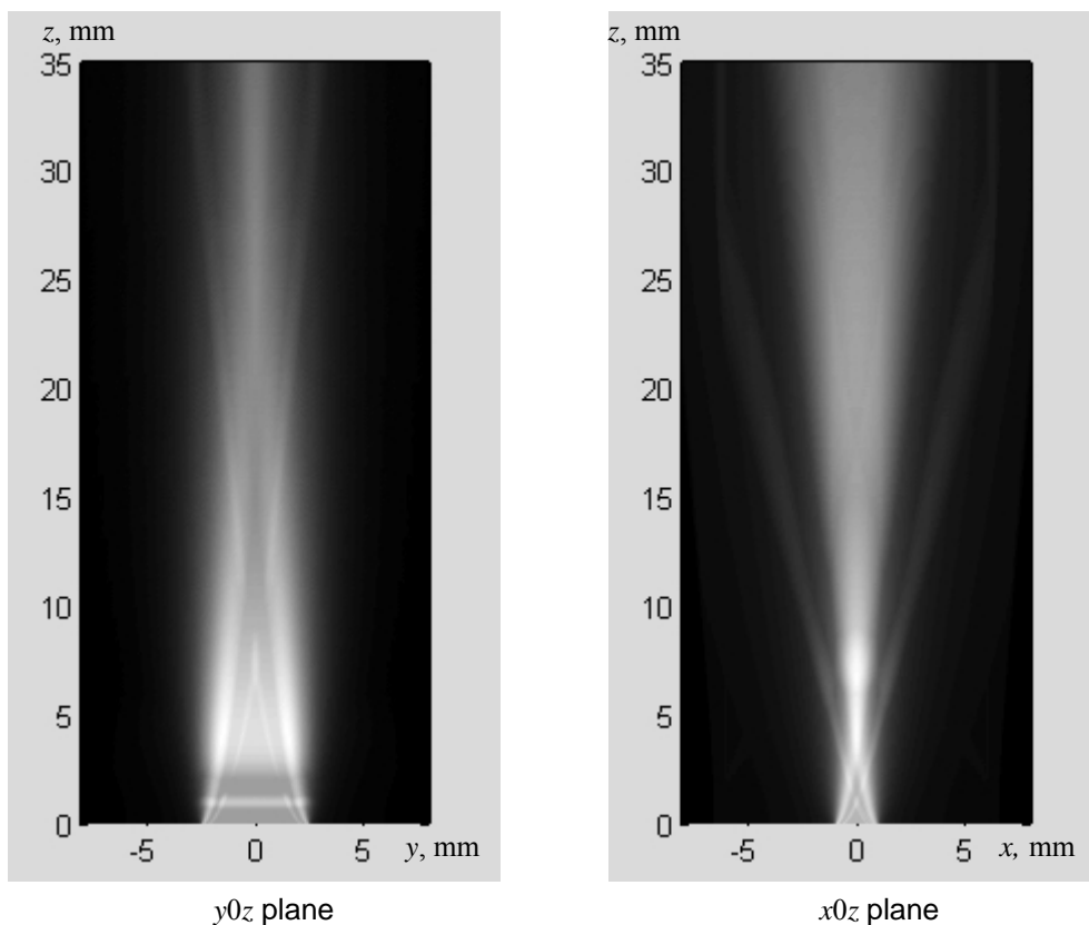
Fig. 5. Ultrasonic field of 5MHz transducer with dimensions 2x5mm
