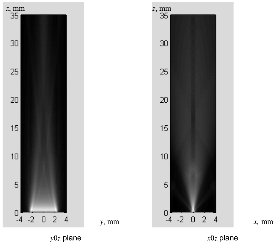
Fig. 10. Ultrasonic fields in a transmission mode of 10 MHz transducer (0.7×5 mm)
