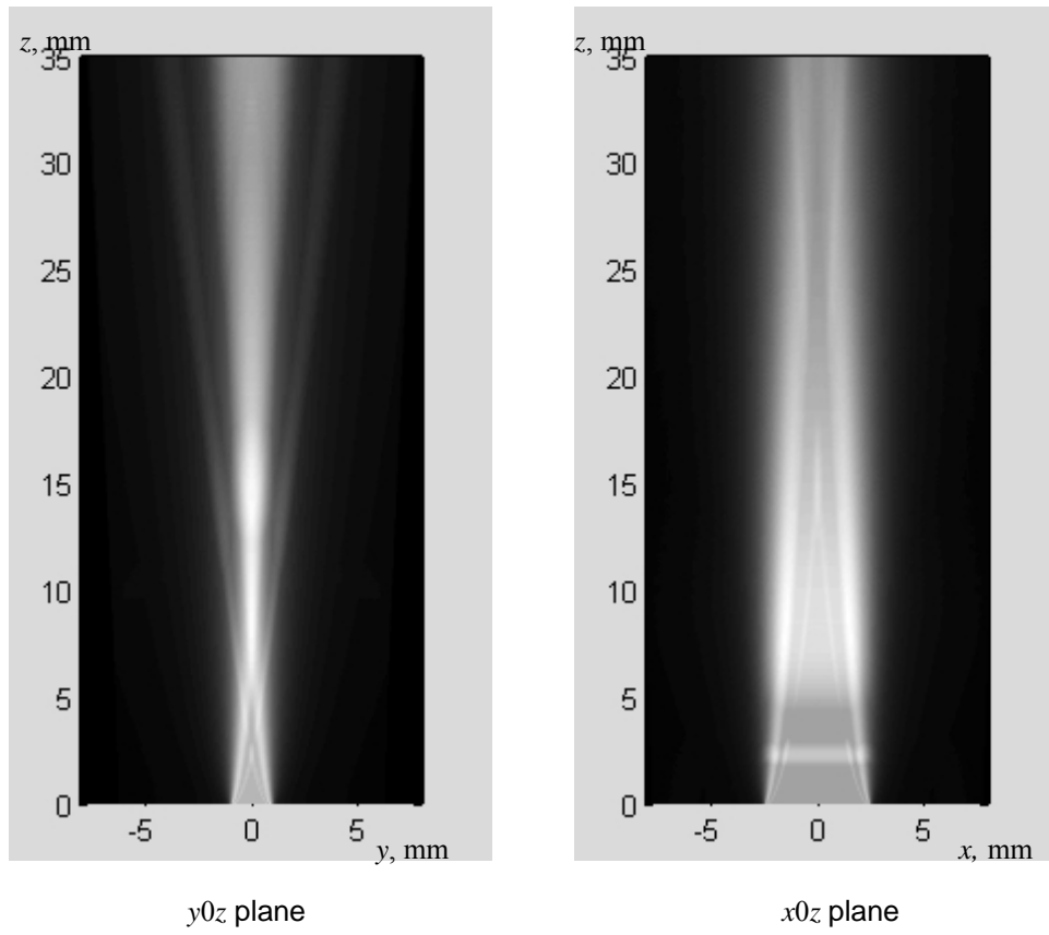
Fig. 8. Ultrasonic fields in a transmission mode of 10 MHz transducer (2×5 mm)
