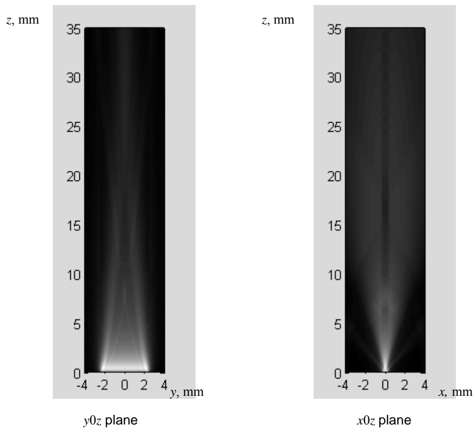
Fig. 7. Ultrasonic field of 5MHz transducer with dimensions 0.7x5 mm
