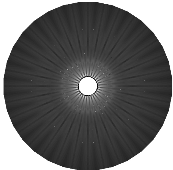
Fig. 12. The coverage of the field of the radial array 5MHz, 5x0.7mm, N=32
