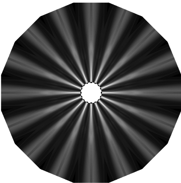
Fig. 11. The coverage of the field of the radial array 10MHz, 5x1mm, N=16
