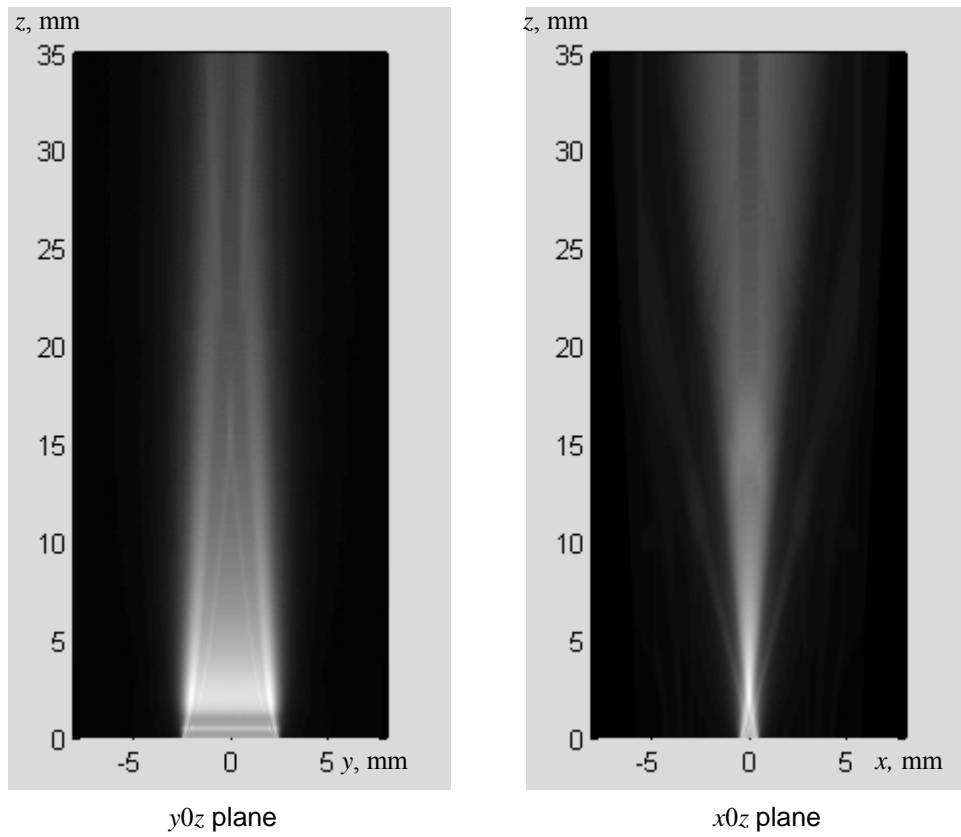
Fig. 9. Ultrasonic fields in a transmission mode of 10 MHz transducer (1×5 mm)
