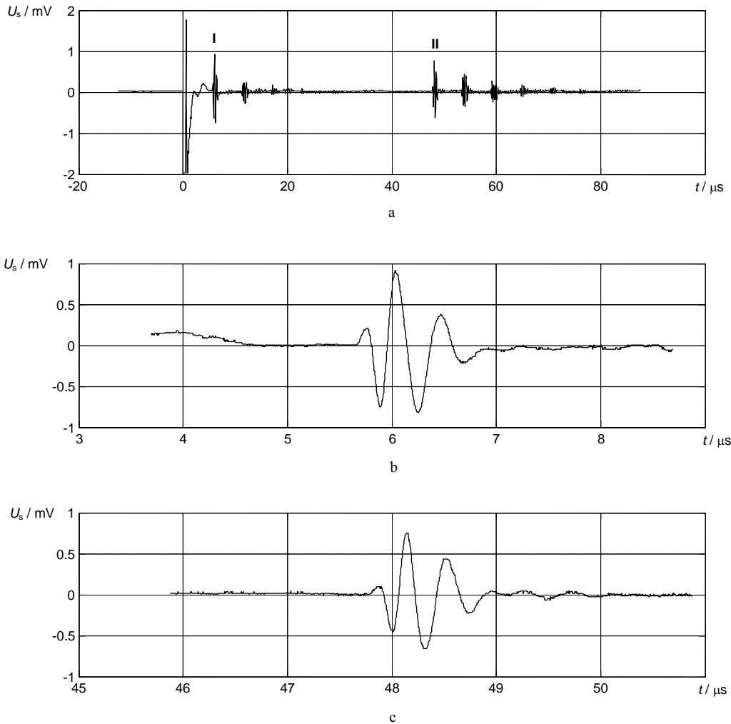
Fig. 5. Experimental signal in a liquid Pb-Bi at the temperature 456^{\circ}\text{C} : a-the full signal; b-the first reflection I from the interface protector/liquid metal and the first reflection II from an aluminum plate in a liquid metal.
