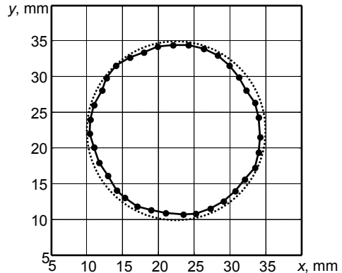
Fig. 12. Cross – sections of amplitude C-scan image of 25 mm delamination type defect at the zone of amplitude maximum. Dotted line is real contour of the 25 mm delamination type defect
