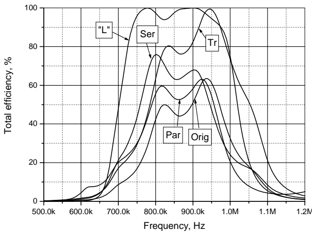
Fig. 15. Total efficiency
