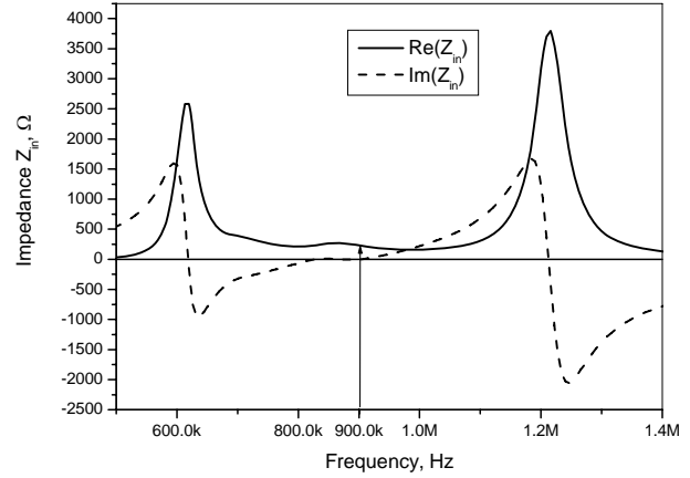
Fig. 5. Impedance after parallel inductance compensation
