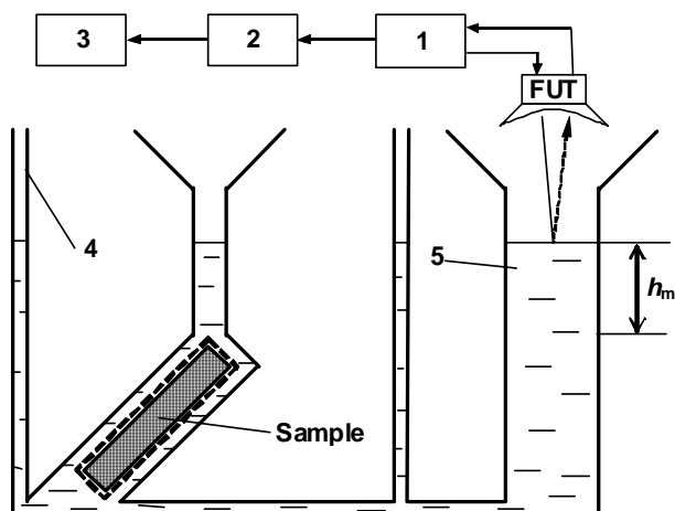
Fig.4. Stages of the porosity evaluation process using the acoustic echolocation method: 1 - the acoustic liquid level meter, 2 - interface, 3 - personal computer, 4 - the reticular case for the sample, 5 - the liquid level measurement part.
