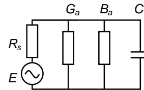
Fig. 5. Equivalent circuit of IDT connected to RF source
