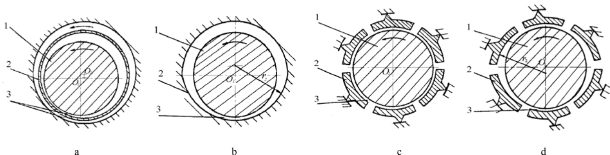
Fig. 1. Bearings : a – self-adjustment including floating ring bearings, b – elliptical bearings, c - tilting-pad journal bearings, d - elliptical tilting pad journal bearings; 1 - rotor, 2 - floating spacer or segment, 3 - carrying lubricating layer
