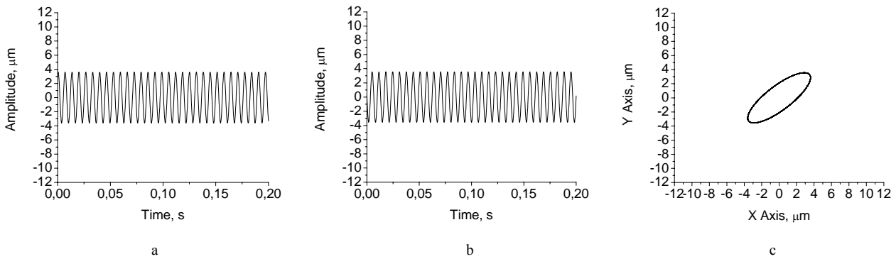
Fig. 6. Adaptive hydrodynamic bearings with elastic ring that is moved easily, when frequency of rotor rotation is 2994 rpm: a – signal of vibrochange in the horizontal direction, b - signal of vibrochange in the vertical direction, c – orbit.
