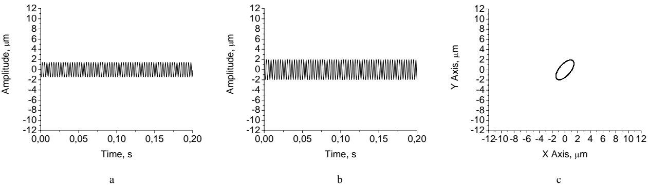
Fig. 7. Adaptive hydrodynamic bearings with several shoulders that are connected segments, when frequency of rotor rotation is 4025 rpm: a - signal of vibrochange in the horizontal direction, b - signal of vibrochange in the vertical direction, c – orbit
