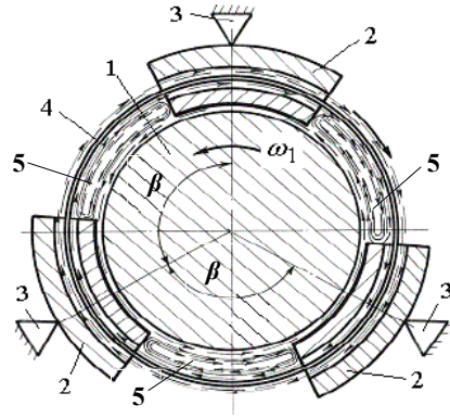
Fig. 4. Adaptive hydrodynamic bearing with elastic ring that is moved easily and is connected segments 1 – rotor, 2 – segments, 3 – adaptive thrust, 4 – elastic ring, 5 – lubricant
