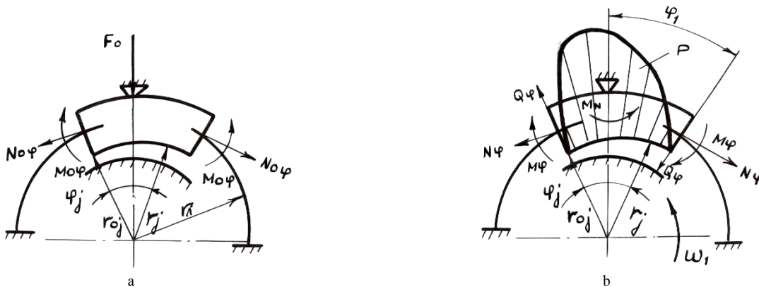
Fig. 3. Powers that are operated on segments of bearing: a – being preconceived weighting, b – being hydrodynamic pressure
