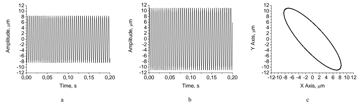
Fig. 8. Adaptive hydrodynamic bearings with elastic ring that is moved easily, when frequency of rotor rotation is 4030 rpm: a - signal of vibrochange in the horizontal direction, b - signal of vibrochange in the vertical direction, c – orbit
