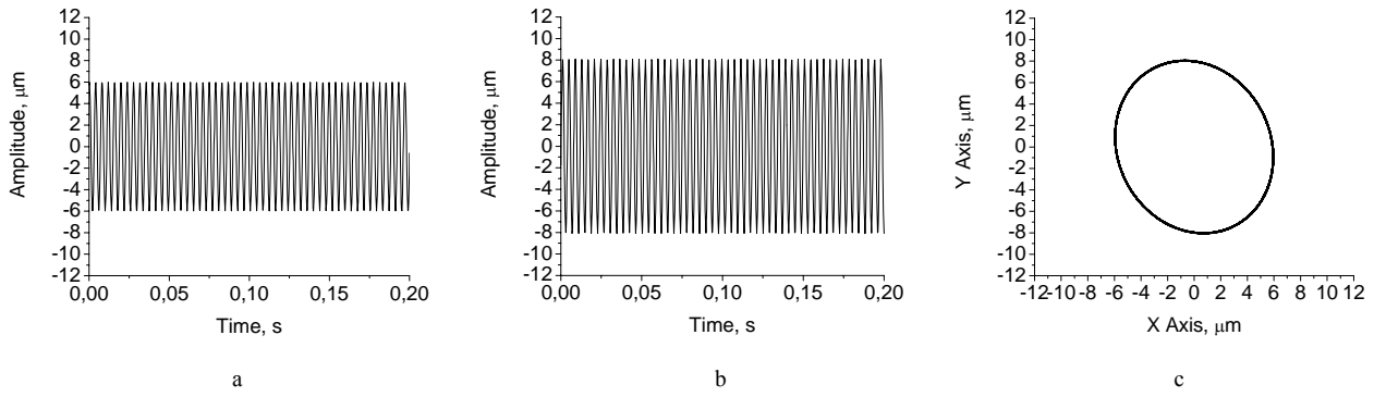
Fig. 5. Adaptive hydrodynamic bearings with several shoulders that are connected segments, when frequency of rotor rotation is 2984 rpm: a – signal of vibrochange in the horizontal direction, b - signal of vibrochange in the vertical direction, c – orbit.
