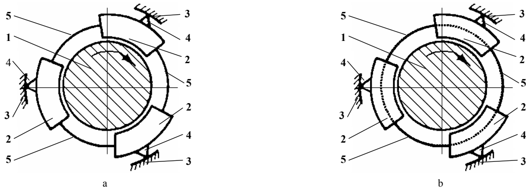
Fig. 2. Adaptive hydrodynamic bearings: a – elastic shoulders that are connected segments: 1 - rotor, 2 – segments 3 - spindle head 4 - adaptive thrust; 5 - elastic shoulders that are connected segments; b – with elastic ring that is moved easily and is connected segments: 1 - rotor, 2 – segments 3 - spindle head 4 - adaptive thrust, 5 - elastic ring
