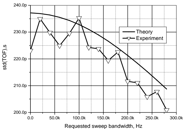
Fig. 12. Unfiltered chirp signal performance
