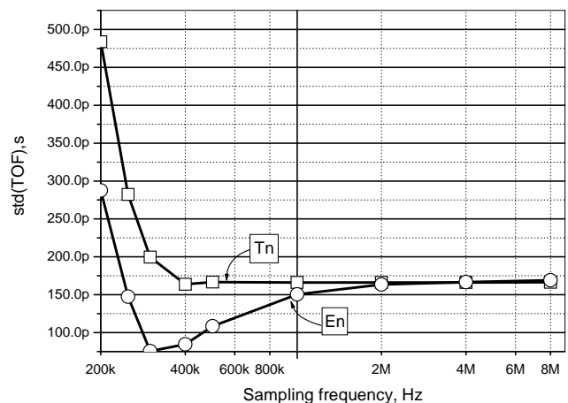
Fig. 9. ToF deviation versus the sampling frequency
