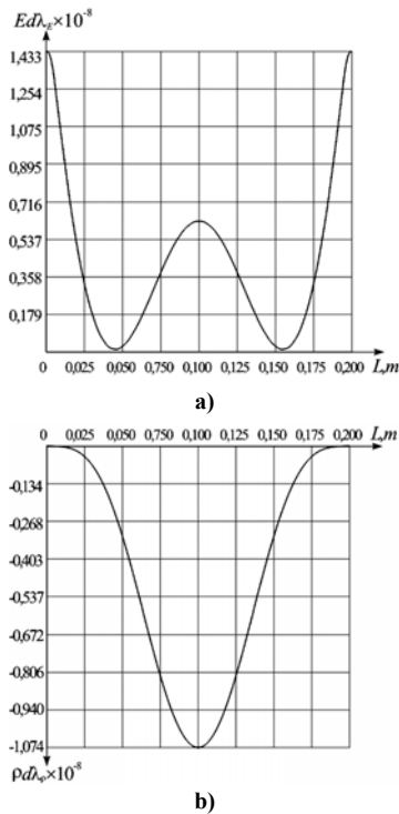
Fig. 1. Effect of the change of: a) modulus of elasticity, b) density to the first eigenvalue
