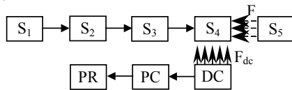
Fig.5. Structural diagram of the setup for experimental investigations: S_1 – signal generator; S_2 – signal amplifier; S_3 – setup for the analysis of vibrations; S_4 – the investigated material; S_5 – source of monochromatic light; DC – digital camera; PC – personal computer; PR – printer; F_{dc} – light flux of the digital camera; F – flux of light projected using the source of light through the grid of the step p at an angle \alpha
