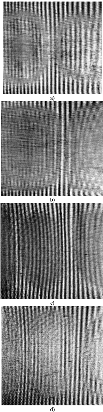
Fig. 8. The second eigenmode of the paper Plano Plus 80 g/m 2 : a) different density of the paper, longitudinal direction of production (frequency of vibrations 158 Hz, amplitude 2 \times 10^{-6} m); b) different density of the paper, transverse direction of production (frequency of vibrations 174 Hz, amplitude 2 \times 10^{-6} m); c) paper without defects, longitudinal direction of production (frequency of vibrations 186 Hz, amplitude 2 \times 10^{-6} m); d) paper without defects, transverse direction of production (frequency of vibrations 180 Hz, amplitude 2 \times 10^{-6} m).
