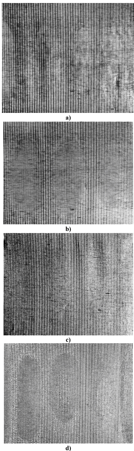
Fig.10. The fourth eigenmode of the paper Plano Plus 80 g/m 2 : a) different density of the paper, longitudinal direction of production (frequency of vibrations 181 Hz, amplitude 2 \times 10^{-6} m); b) different density of the paper, transverse direction of production (frequency of vibrations 188 Hz, amplitude 2 \times 10^{-6} m); c) paper without defects, longitudinal direction of production (frequency of vibrations 200 Hz, amplitude 2 \times 10^{-6} m); d) paper without defects, transverse direction of production (frequency of vibrations 205 Hz, amplitude 2 \times 10^{-6} m).
