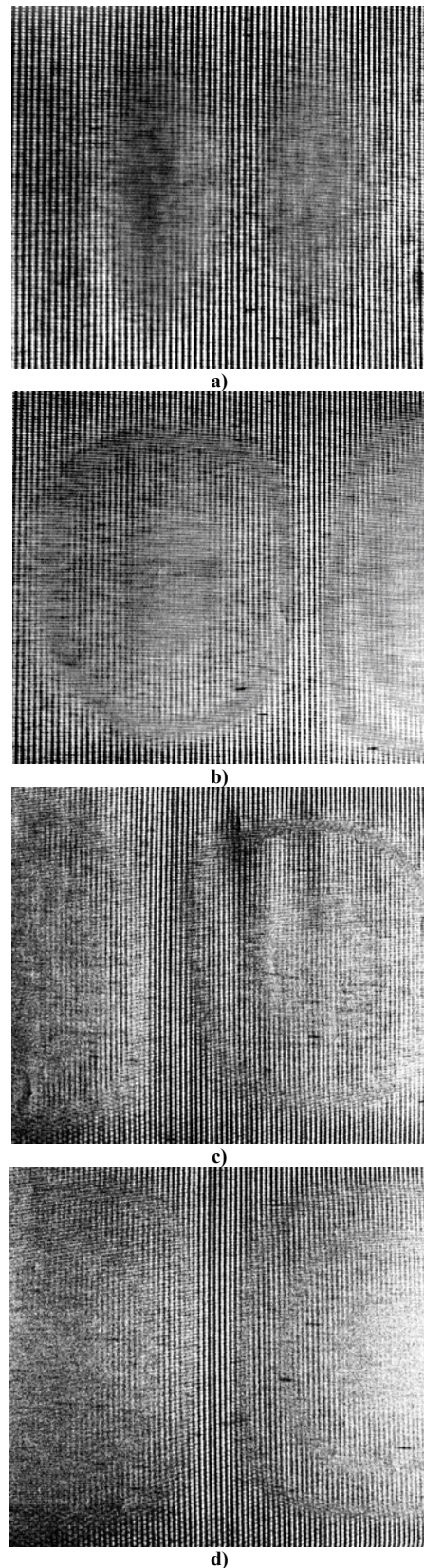
Fig. 7. The first eigenmode of the paper Plano Plus 80\ \text{g/m}^2 : a) different density of the paper, longitudinal direction of production (frequency of vibrations 155\ \text{Hz} , amplitude 2 \times 10^{-6}\ \text{m} ); b) different density of the paper, transverse direction of production (frequency of vibrations 156\ \text{Hz} , amplitude 2 \times 10^{-6}\ \text{m} ); c) paper without defects, longitudinal direction of production (frequency of vibrations 162\ \text{Hz} , amplitude 2 \times 10^{-6}\ \text{m} ); d) paper without defects, transverse direction of production (frequency of vibrations 163\ \text{Hz} , amplitude 2 \times 10^{-6}\ \text{m} ).
