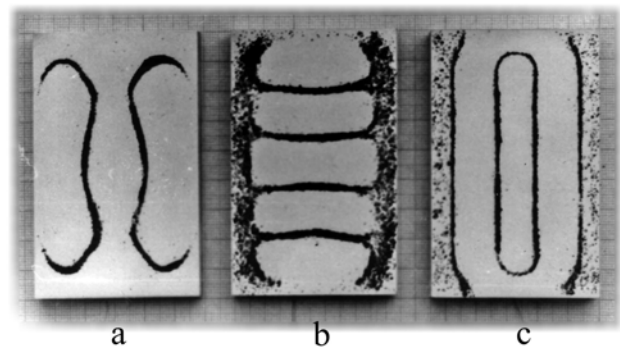
Fig. 5. Chladni figures on the surface of the transducer (Fig. 3), consisting of an aluminum plate (measuring 81.0x44.0x1.0 mm) and a piezoelectric ceramic plate (measuring 60.0x20.0x1.0 mm): a – frequency is 7.09 kHz; b – frequency is 16.89 kHz; c – frequency is 19.03 kHz
