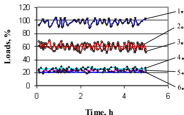
Fig. 5. Work parameters of the defibrator, when consumption of steams is 1.5 t/h: 1 - load of the main electromotor (9); 2 - speed of upper screw (1); 3 - speed of lower screw (4); 4 - load of upper screw (1); 5 - electromotor load of the first screw (8); 6 - electromotor load of the second screw (8)
