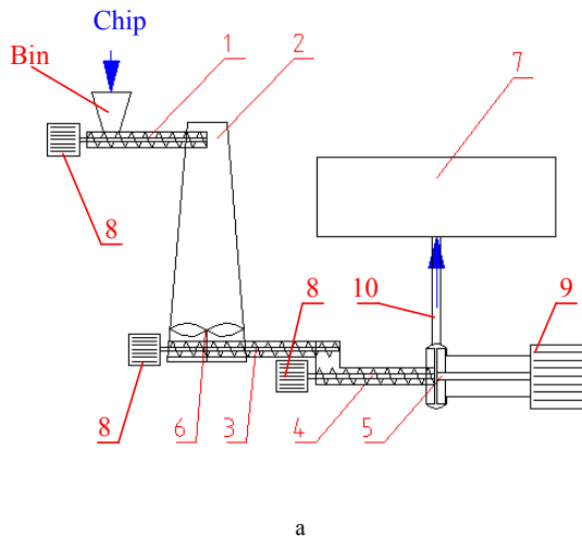
Fig. 2. Object of investigation: a- principle scheme, 1 – screw of supply of steaming camera, 2 – steaming camera, 3 – the first screw of supply, 4 – the second screw of supply grinding camera, 5 – camera with two discs, 6 – stirrer, 7 – reservoir of defibrating mass, 8 – electromotor, 9 – electromotor, 10 – tube of exhaust, b – computer – based scheme in the monitor screen.
