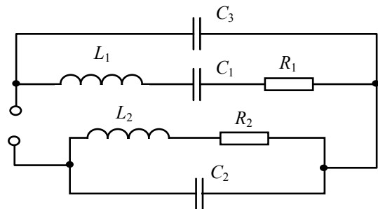
Fig. 2. Equivalent electric diagram of EAT-19 (3ИИ-19) transducer
