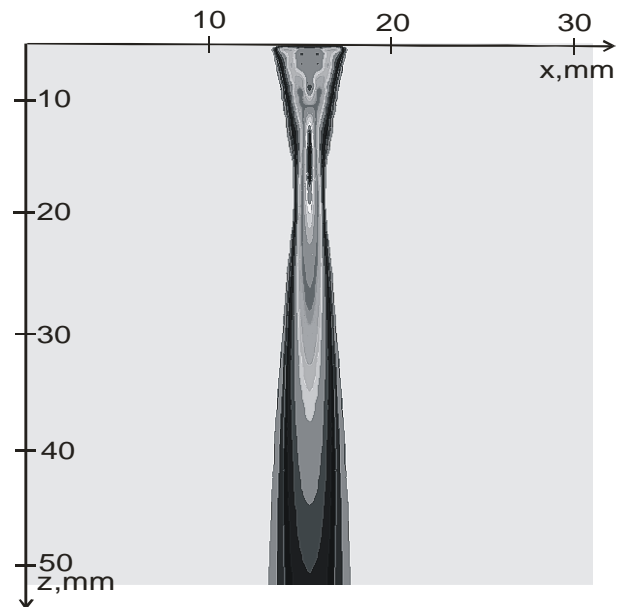
Fig.4. Ultrasonic field of the cylindrical array in xOz plane. N=32 elements are exited at the center frequency f=5 MHz while the beam is focused at the focal distance z_f=15
