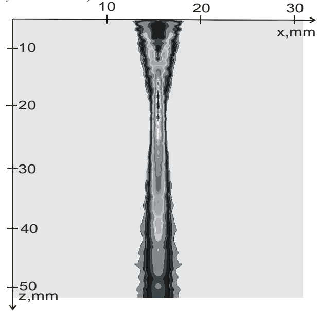
Fig.3. Ultrasonic field of the cylindrical array in xOz plane. N=48 elements are exited at the center frequency f=5 MHz while the beam is focused at the focal distance z_f=20 mm
