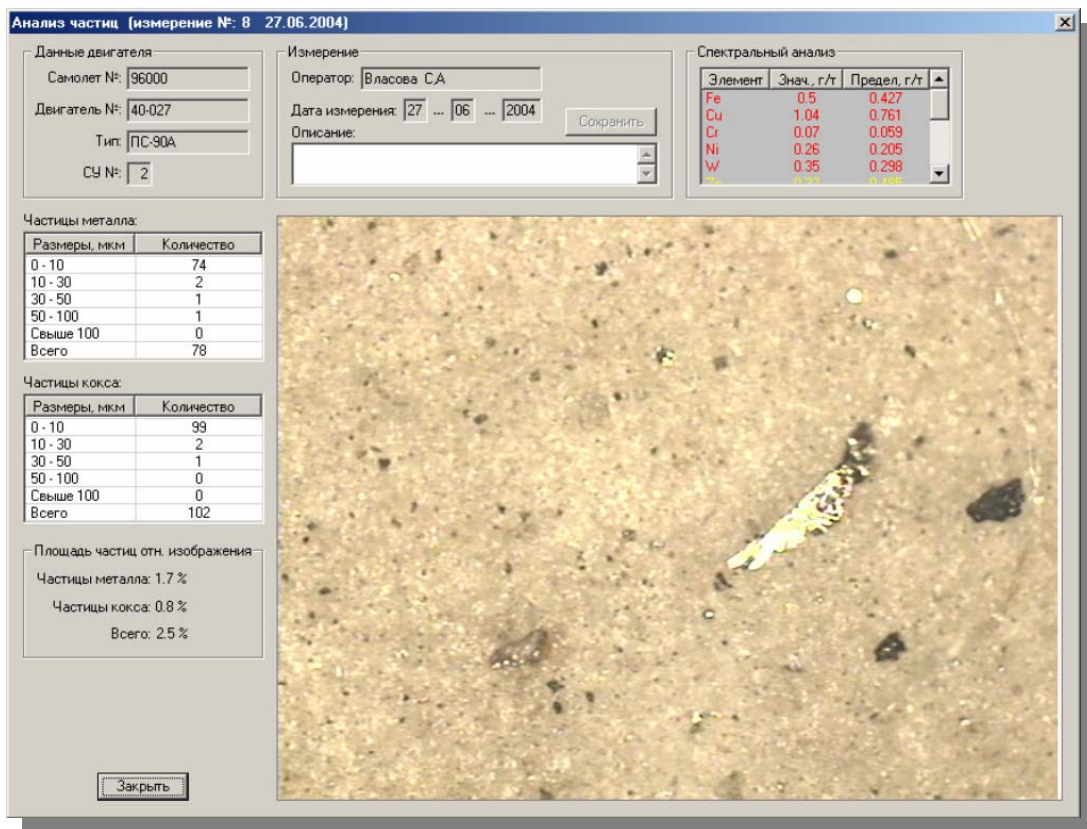
Fig.2. Analysis of the particles wear
