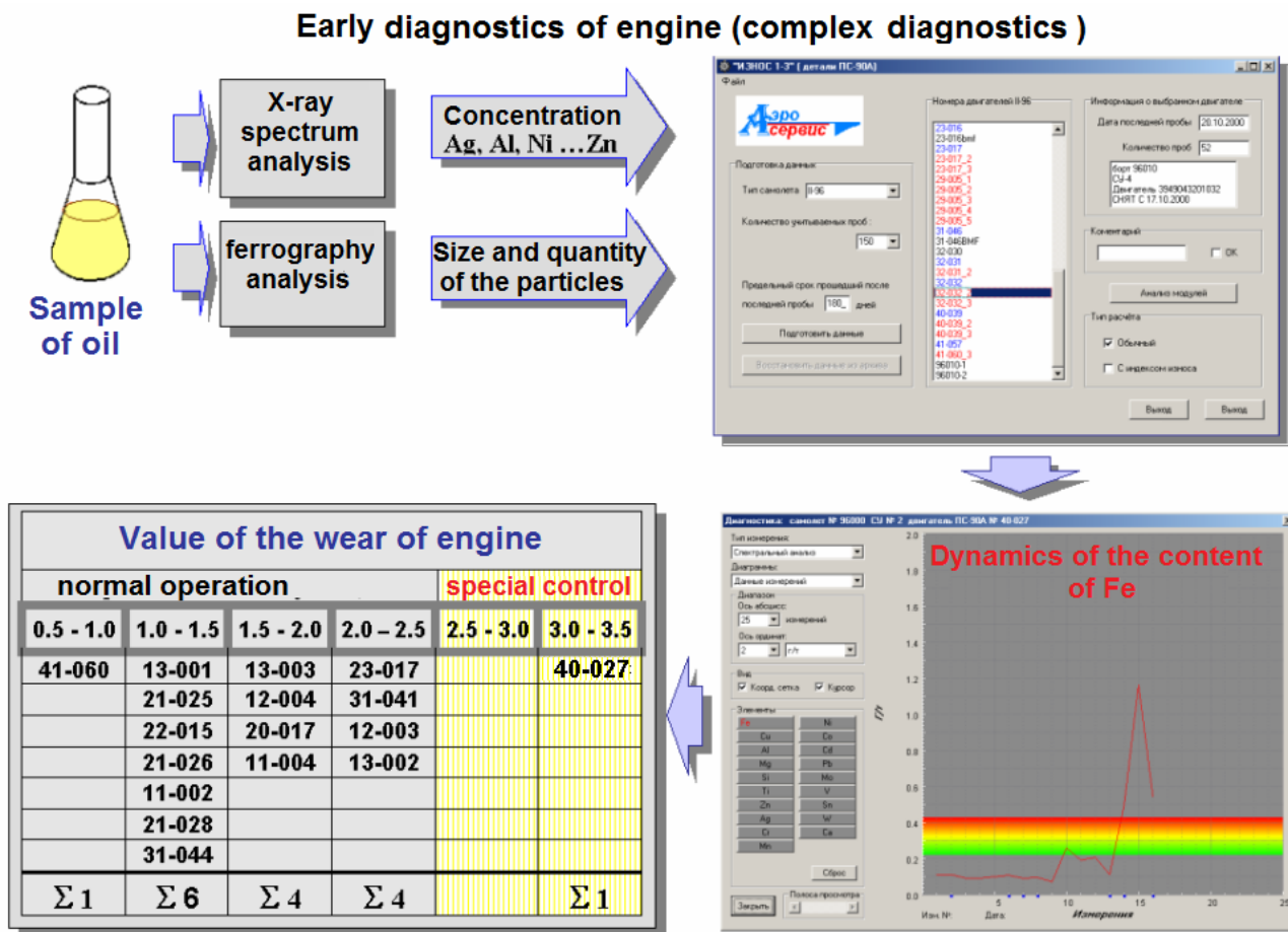
Fig. 1. The structural scheme of the organization of the work (researches) in the tribomonitoring field
