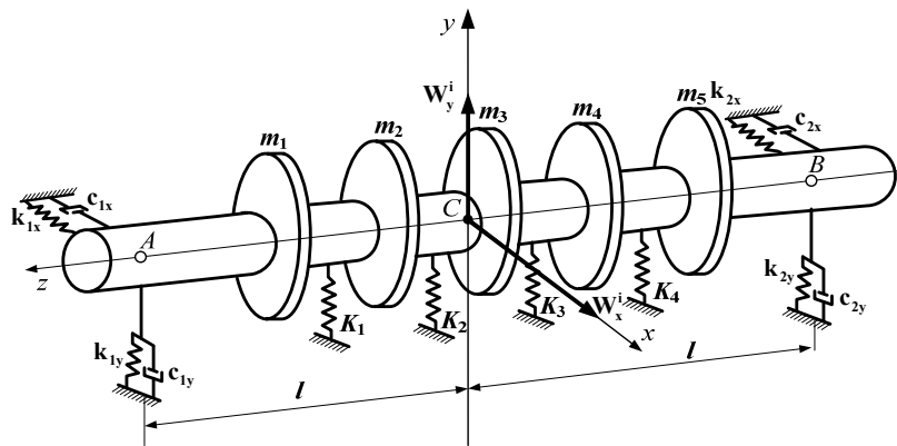
Fig. 8. Dynamical model of centrifugal pump with discs
