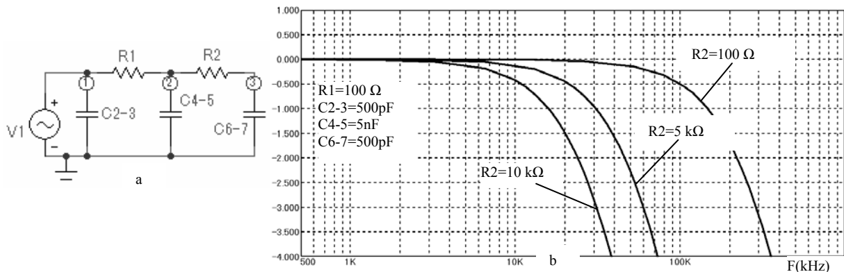
Fig. 9. Equivalent circuit and AFR of the transducer (Fig. 5d): a - the equivalent circuit, b - the amplitude-frequency responses at various values of the resistance R_2 at R_1=100\Omega , C_{2-3}=500pF , C_{4-5}=5nF , C_{6-7}=500pF
