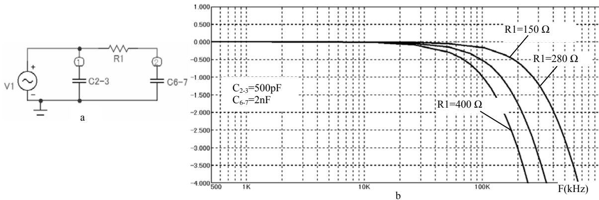
Fig. 8. Equivalent circuit and AFR of the transducer (Fig. 5c): a - the equivalent circuit, b - the amplitude-frequency responses at various values of the resistance R_1 at C_{2-3}=500pF , C_{6-7}=2nF
