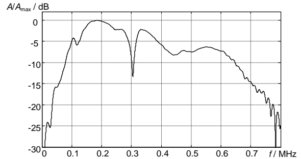
Fig. 14. The frequency response of the transducer with the convex protector (the equivalent diameter of the contact area 3 mm)
