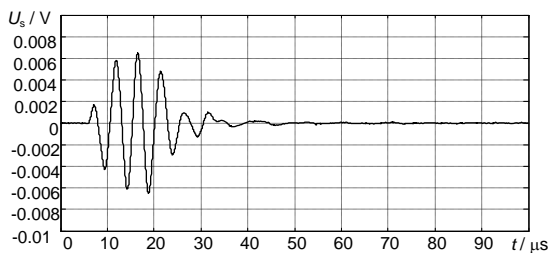
Fig. 13. The ultrasonic signal of the transducer with the convex protector (the equivalent diameter of the contact area 3 mm)
