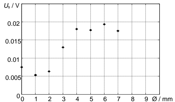
Fig. 15. The dependence of the amplitude of the ultrasonic signal in the case of convex protectors with different diameters of the contact area
