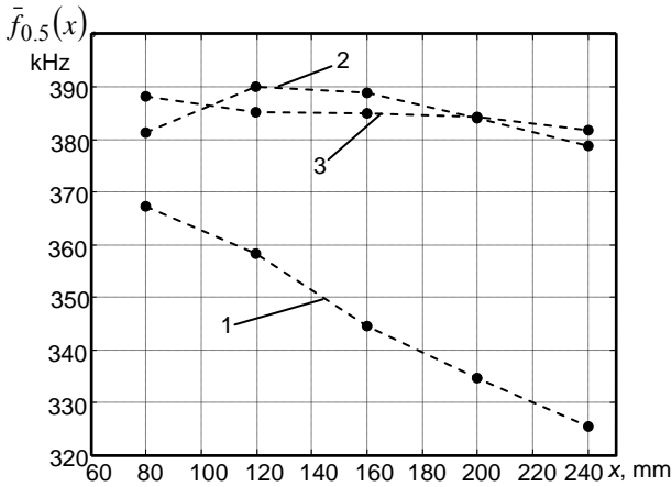
Fig.14. The equivalent frequencies of different half periods of the S_0 mode signal versus distance from the transmitter obtained using different zero-crossing instants in the measured experimental signals
