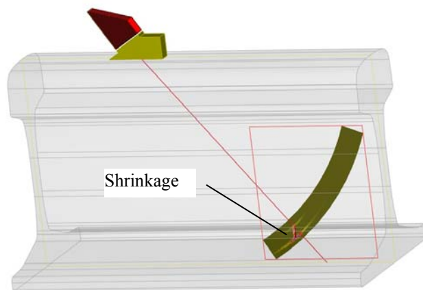
Fig. 20. Defect response superimposed on the rail sample in 3D
