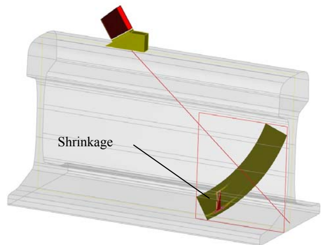
Fig.17. Defect response superimposed on the rail sample in 3D
