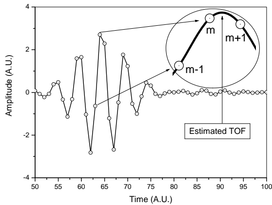
Fig. 1. Parabolic interpolation for TOF estimation [23]
