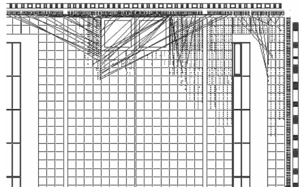
Fig. 6. Filter logic placement on FPGA die
