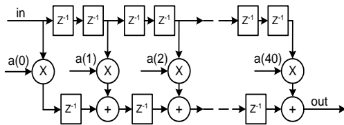
Fig. 3. Filter configuration used
