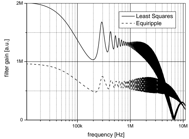
Fig. 5. FIR filters AC response
