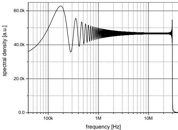
Fig. 4. Test signal spectrum
