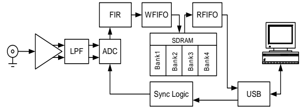
Fig. 2. The experimental system structure (hardware setup)
