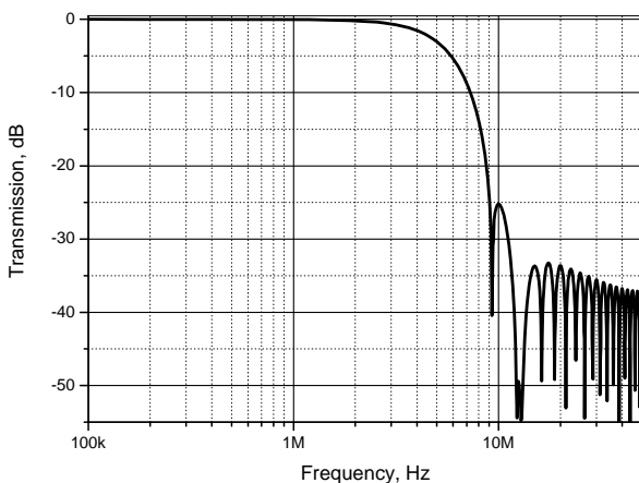
Fig. 10. Filter AC response
