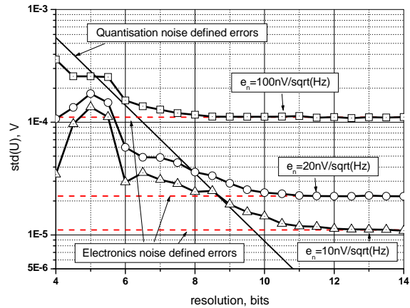
Fig. 8. Amplitude estimation errors vs. ADC resolution
