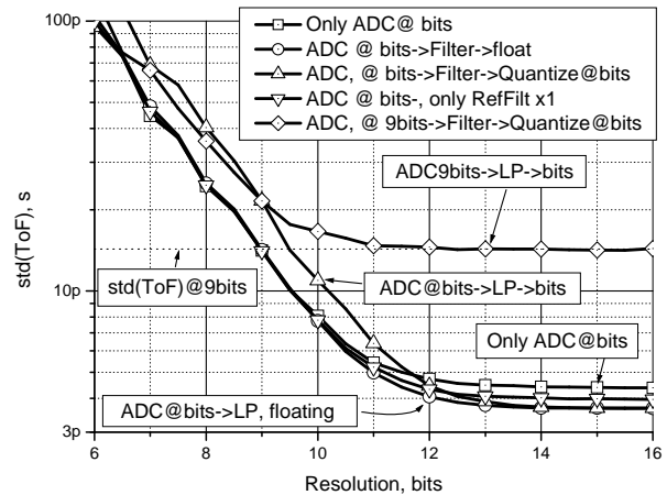
Fig. 11. TOF variance vs. ADC and filter output resolution
