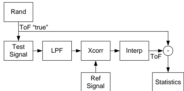
Fig. 9. TOF numerical simulation experiment structure
