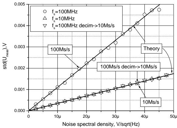
Fig. 7. Voltage standard deviation vs. noise spectral density
