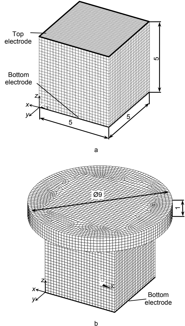
Fig. 1. Graphical representation of the finite element model of piezoelectric transducer: a - piezoceramic cube, b - piezoceramic cube with front matching layer
