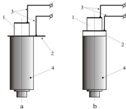
Fig. 4. The schemes of the investigation of the low frequency transducers: a – 1 – piezoelement, 2 – contact layer, 3 – connecting wires, 4 – broadband piezotransducer; b – 1 – piezoelement, 2 – matching layer, 3 – connecting wires, 4 – broadband piezotransducer.
