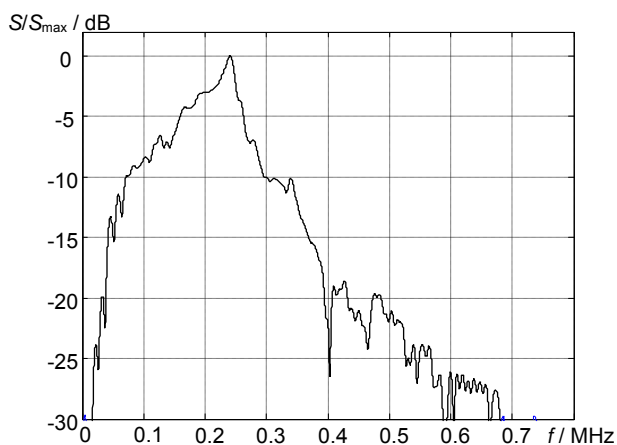
Fig. 7. The ultrasonic signal of the broadband transducer and the piezoelement with matching layer having thickness of 1 mm
