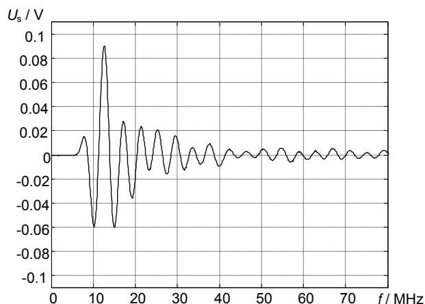
Fig. 8. The frequency response of the transmitter – receiver of the cube piezoelement with the matching layer
