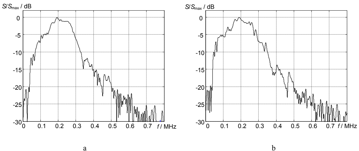
Fig. 11. The frequency response of the receiver-transmitter: a – the single cube (receiver), b – the cube (receiver) with the matching layer
