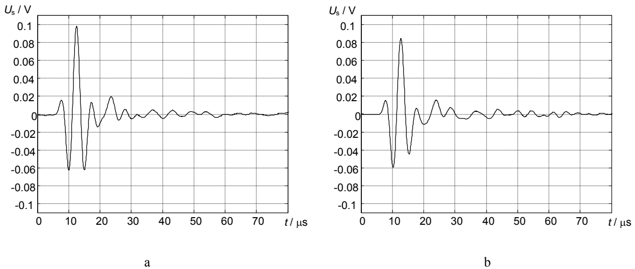
Fig. 10. The ultrasonic signals: a – without matching layer, b – with matching layer
