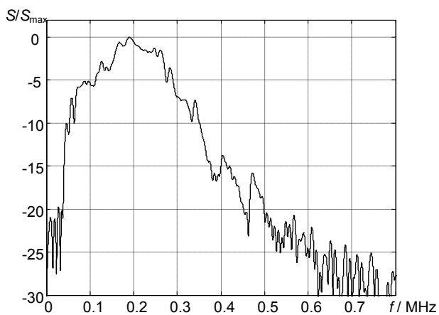
Fig. 6. The frequency response of the transmitter – receiver of the single cube
