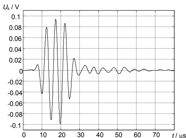
Fig. 9. Ultrasonic signal when the piezoelement was acting as the receiver
