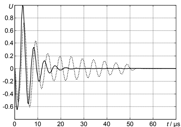
Fig. 3. Normalized time diagrams of the particle velocities at the surface of the ultrasonic transducer. The solid line - piezoceramic cube, the dotted line - piezoceramic cube with the front matching layer
