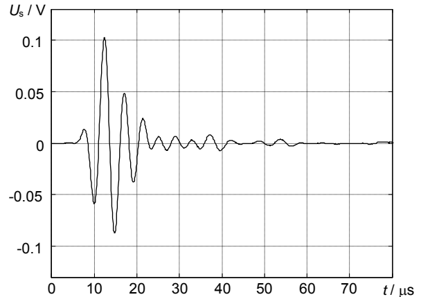
Fig. 5. The received ultrasonic signal in the case than the piezoelement was used as the transmitter.
