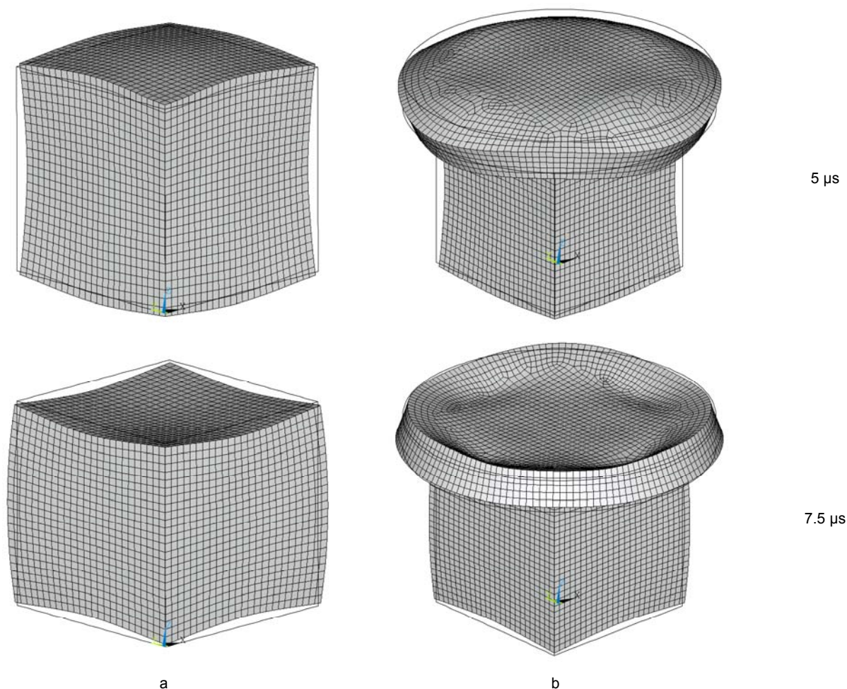
Fig. 2. Displacements of the piezoceramic cube (a) and piezoceramic cube with fibreglass front matching layer (b) oscillating in vacuum at the different instants of time
