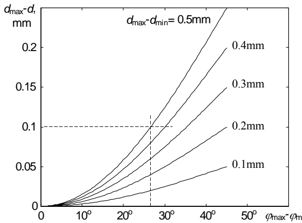
Fig.3. The differences between the maximal diameter d_{max} and measured diameter d when the angle between them is \phi_{max} - \phi_m , for the various cases of the ellipsity of the tube d_{max} - d_{min} .
