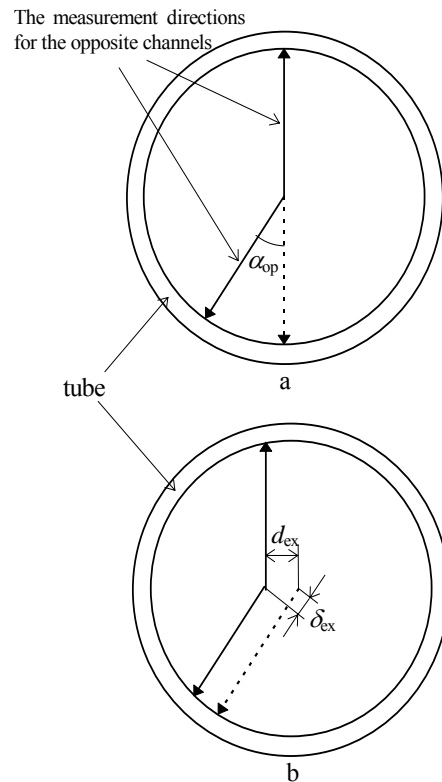
Fig.2. Explanation of dynamic errors
