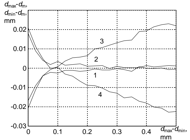
Fig.4. The mean values of the errors if the approximation is used(1,2) and if not used (3,4). 1,3 - for minimal diameter, 2,4 - maximal diameters.
