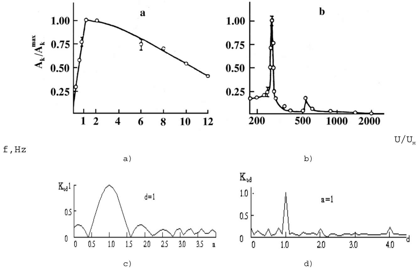
Fig.6. Comparison of results of experimental and mathematical modeling: a),b) - experimental curves; c),d) - calculated curves
