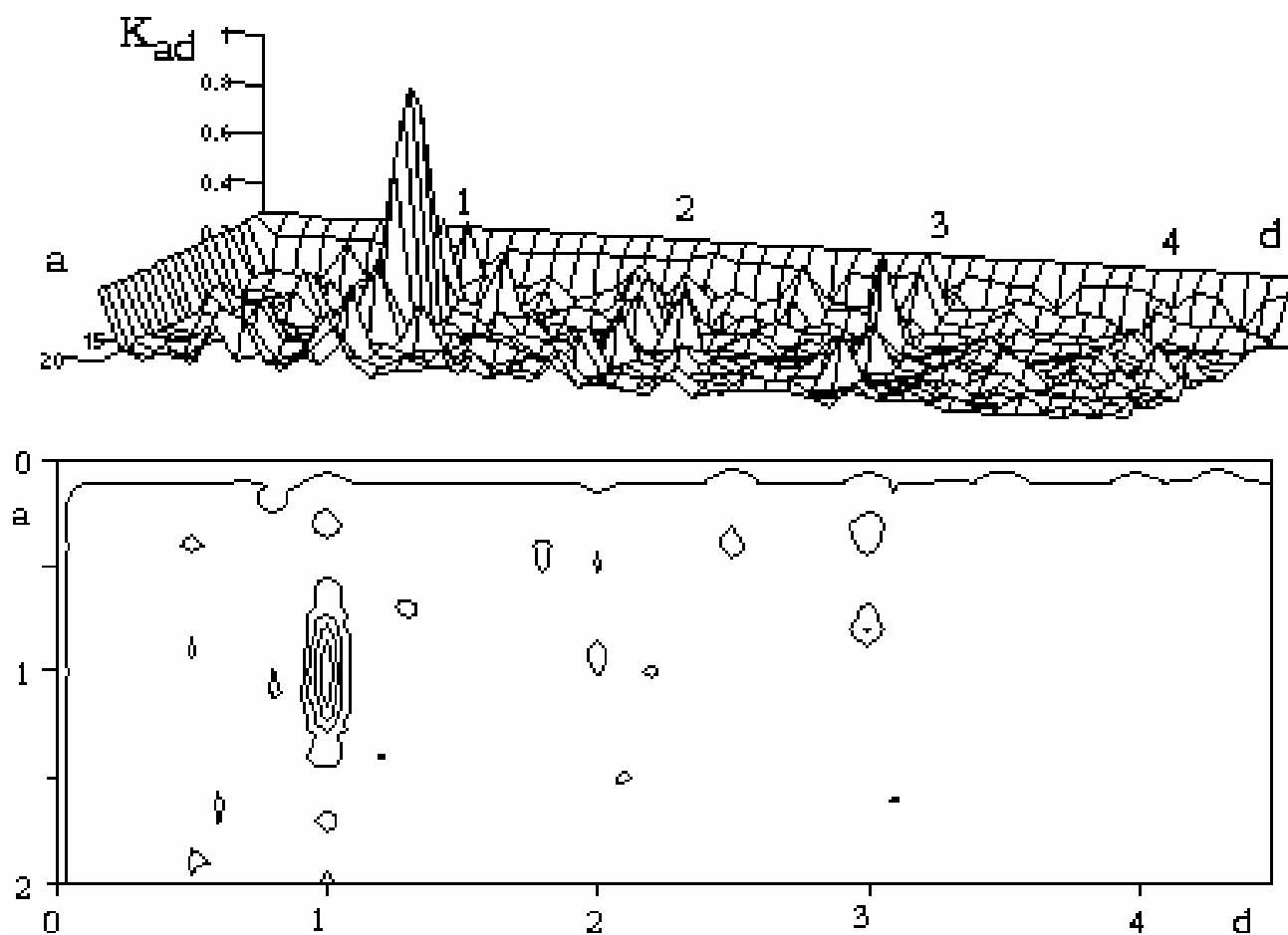
Fig.4. Amplitude - frequency filtering characteristics when microrelief M(x)=\sin(2\pi,4,x) is evaluated
