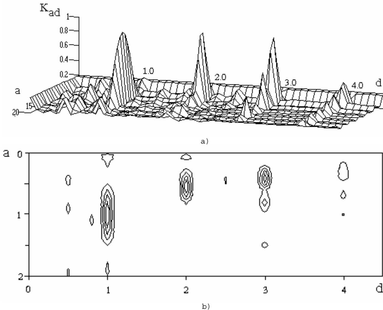
Fig.2. Amplitude - frequency filtering characteristics: a) - surface graph, b) - contour graph
