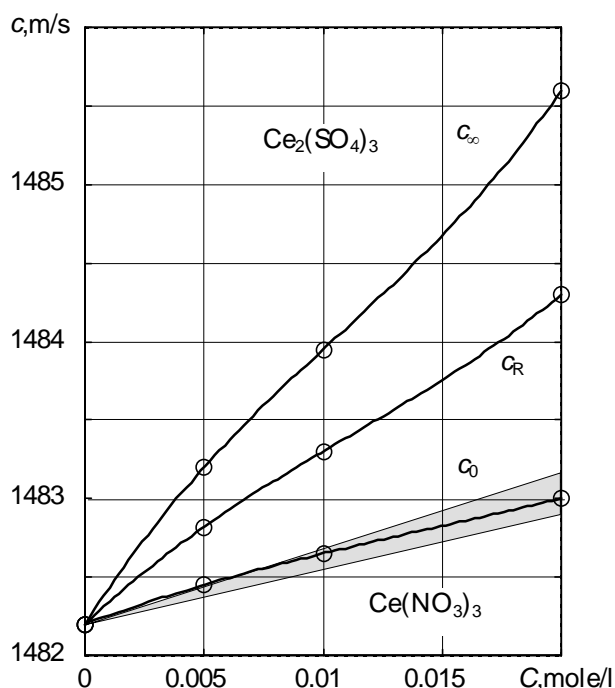
Fig.2. Ultrasound velocity dependence on concentration in Ce_2(SO_4)_3 and Ce(NO_3)_3 solutions at 20°C
