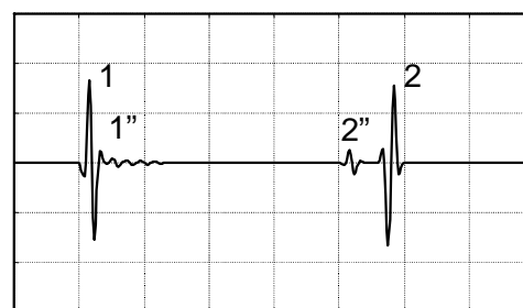
Fig. 4. Additional reflections of short ultrasonic pulse from the clot separated from the cell walls
