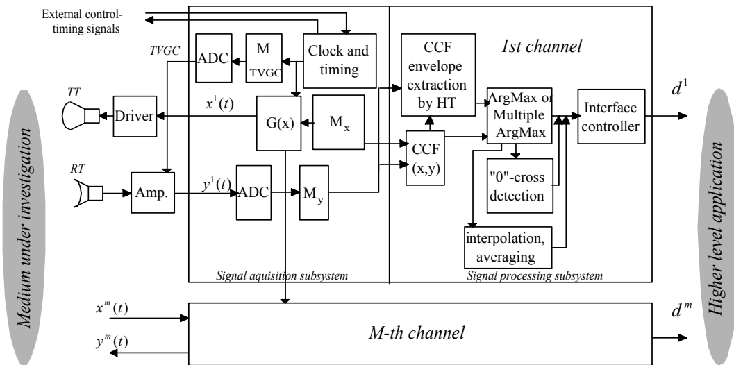
Fig. 1. CDFG of the general TDE task.
