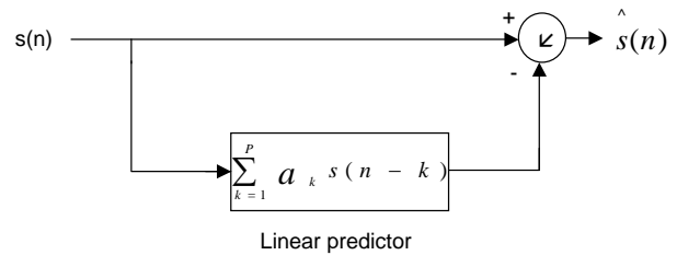
Fig. 1: Inverse filter
