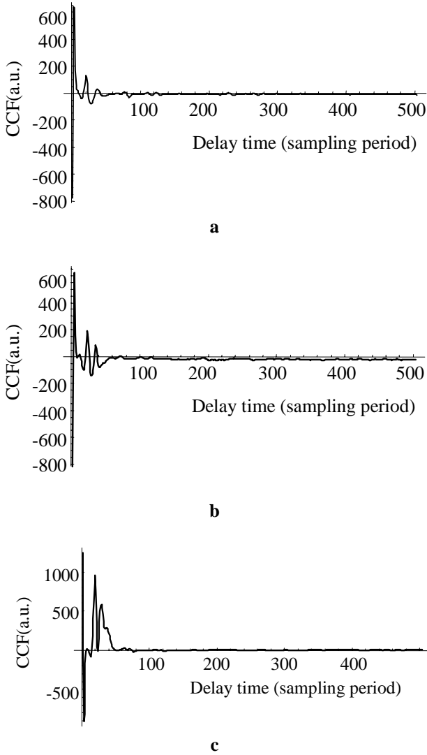
Fig. 4. Multi target detection (a) CCF for the first position 'A' of the receiver (b) CCF for the 2nd position 'B' of the receiver (c) CCF for the 3rd position 'C' of the receiver
