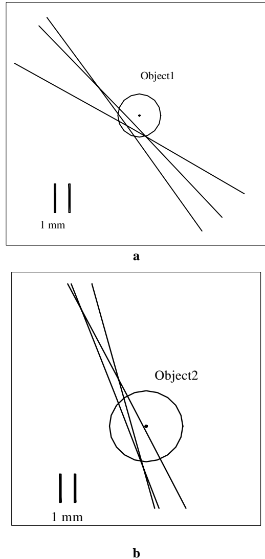
Fig. 6. A magnified view of the actual object location and the points of coincidence of the ellipsoids in Fig. 4, (a) Actual location of object 1 (b) Actual location of object 2
