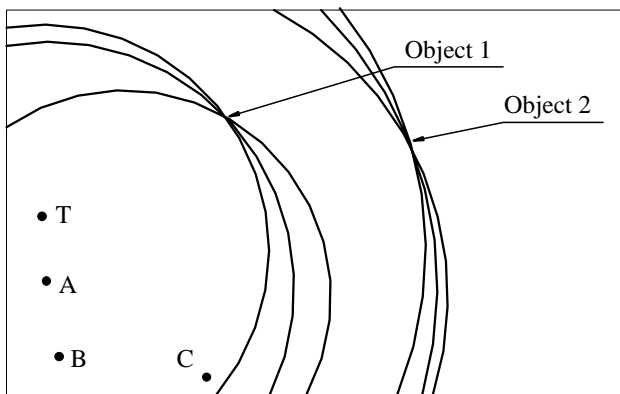
Fig. 5. Determination of the object location
