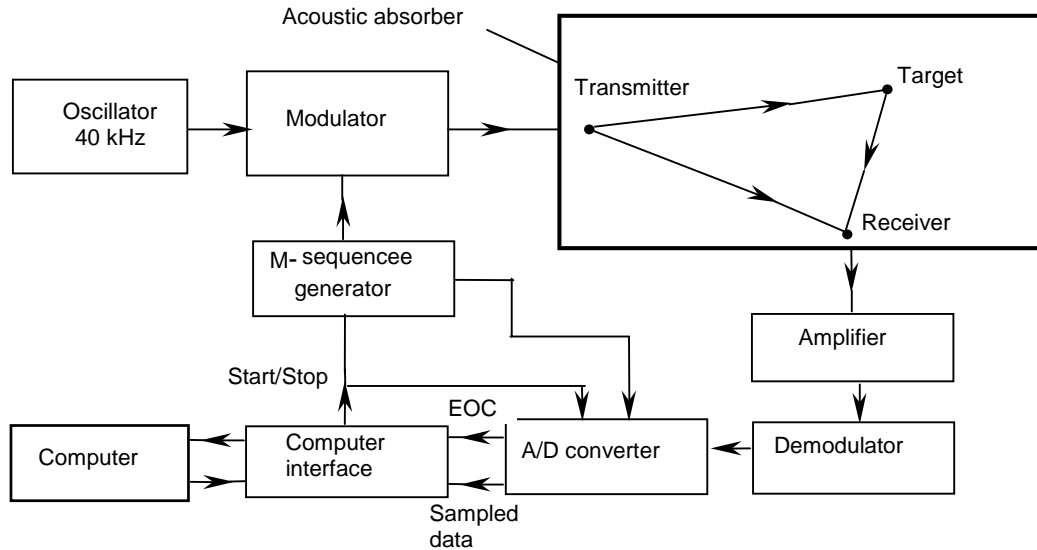
Fig. 2. Block diagram of the experimental setup
