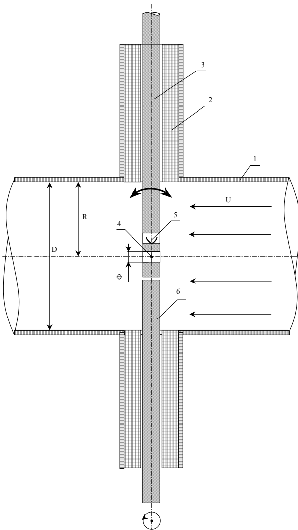
Fig.6. Experimental arrangement for measurement of the axial directivity pattern: 1- pipe, 2- mounting system of the transducer with the mock-up of an ultrasonic transducer, 3- housing of the thermo anemometer, 4- flow-sensing element, 5- thermometer, 6- compensation bar
