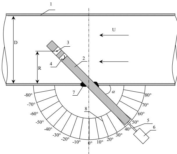
Fig.4. Experimental setup
