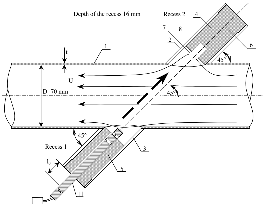
Fig.15. Flow velocity measurement in the acoustical channel
