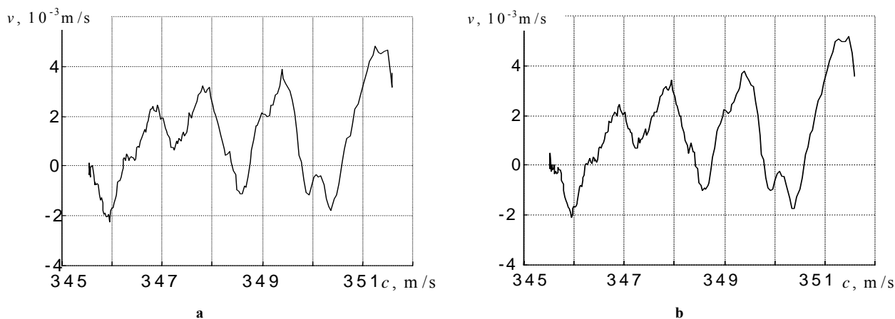
Fig.10. The change of zero drift of the ultrasonic system in two days period when the sound velocity (temperature) in the spoolpiece is changed
