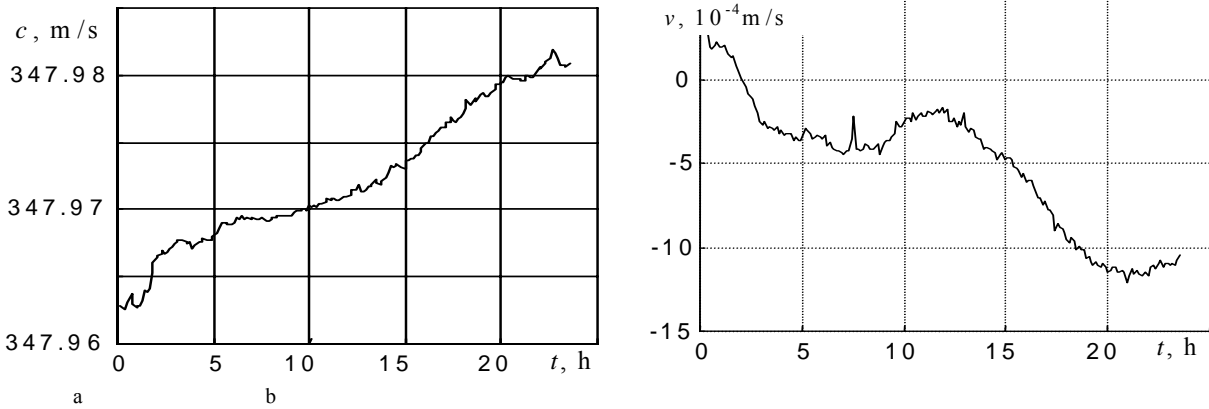
Fig.7. The change of sound velocity-a) and zero drift of the system-b) when the temperature of the spoolpiece was stabilized
