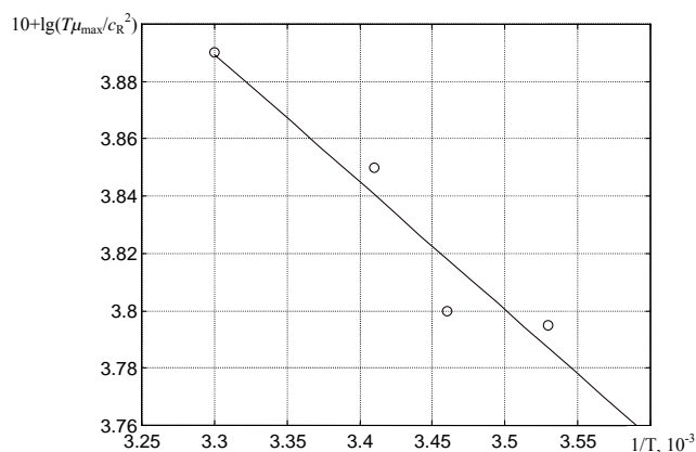
Fig. 3. Graphic determination of the change in the internal energy \Delta H_0 of the relaxation process in MnSO_4 solution
