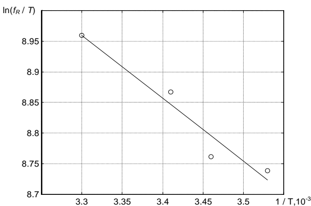
Fig. 1. Variation of \ln(f_R / T) versus 1 / T for MnSO_4 solution
