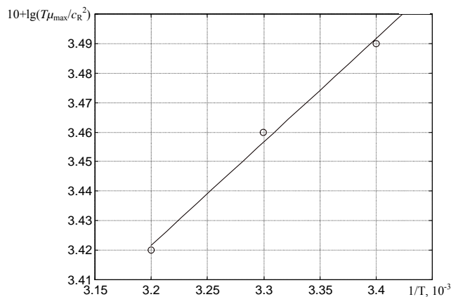
Fig. 4. Definition of the difference in enthalpy \Delta H_0 for complexation reaction in Ln_2(SO_4)_3 solutions
