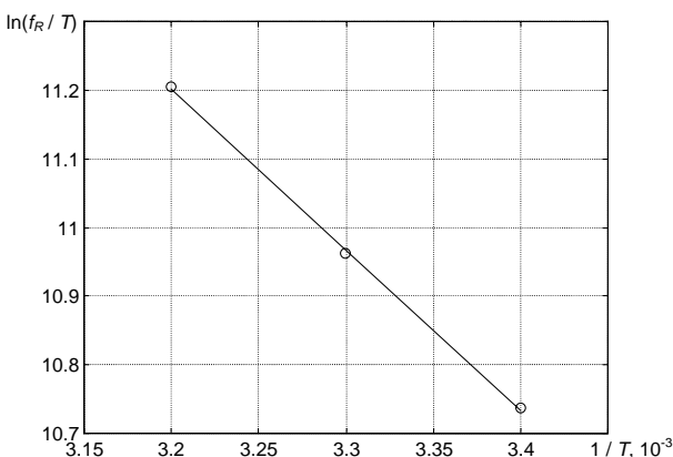
Fig. 2. Variation of \ln(f_R / T) versus 1 / T for Ln_2(SO_4)_3 solution
