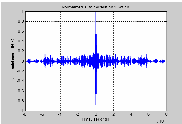
Fig.2. Normalized auto correlation function of the non optimized Short Kasami sequence, the sequence length 63 elements
