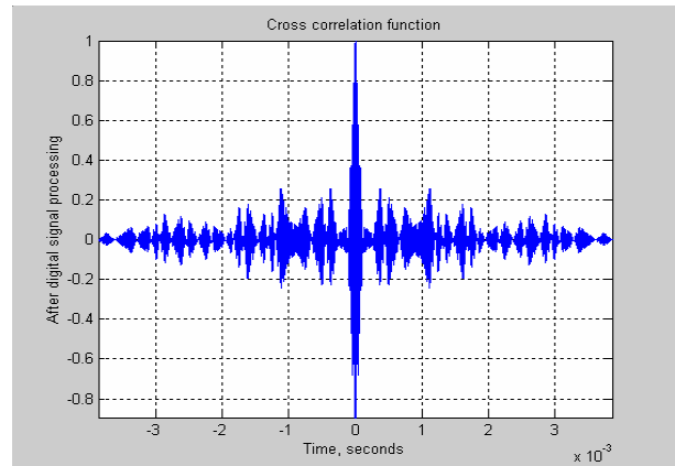
Fig.13. Normalized cross correlation function between the mixture of 60 PN- signals and the reference signal after digital signal processing
