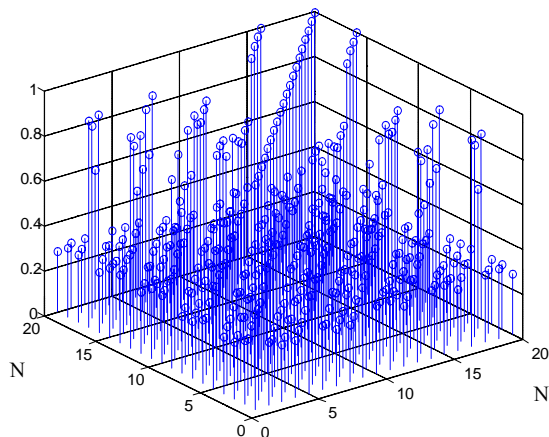
Fig.6. Normalized maximal cross correlation values between the optimized Gold sequences, all sequences are from the same family set: N is the sequence number, the length of sequences is 63 elements
