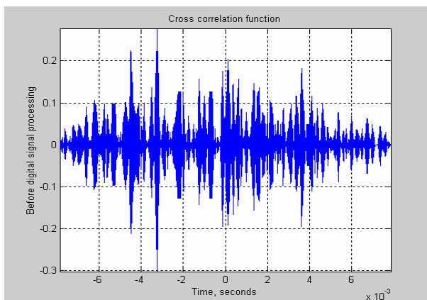
Fig.8. Normalized cross correlation function between the mixture of PN signals and the reference signal before digital signal processing. Signal is calculated summing up 10 PN code sequences
