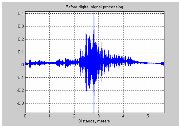
Fig.18. Normalized cross correlation function between the mixture of PN- signals and the reference signal before digital signal processing
