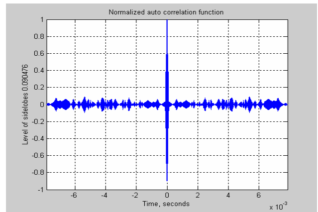
Fig.3. Normalized auto correlation function of the optimized Short Kasami sequence, the sequence length 63 elements
