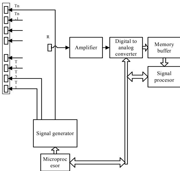
Fig.1. Generic block diagram of ultrasonic multi-channel distance measurement system: T_1 - T_n are transmitters, R is a receiver of ultrasonic waves
