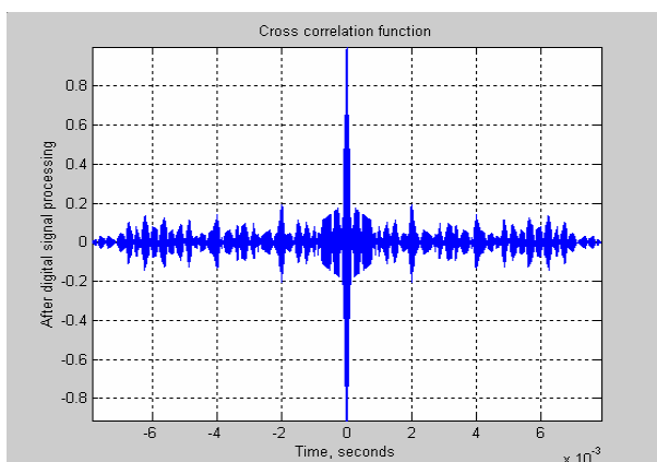
Fig.10. Normalized auto correlation function of the reference signal
