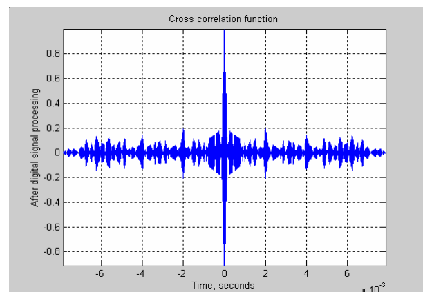
Fig.9. Normalized cross correlation function between mixture of PN signals and the reference signal after digital signal processing. Mixture of signals is calculated summing up 10 PN code sequences
