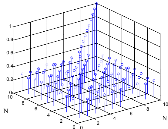
Fig.7. Normalized maximal cross correlation values between the optimized Short Kasami sequences, all sequences are from the same family set: N is the sequence number, the length of sequences is 63 elements
