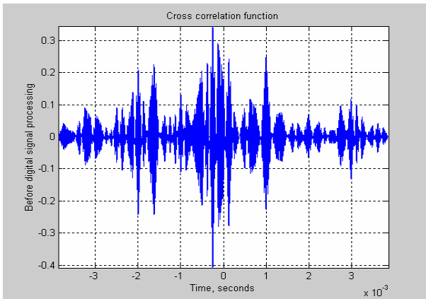
Fig.12. Normalized cross correlation function between the mixture of 60 PN- signals and the reference signal before digital signal processing
