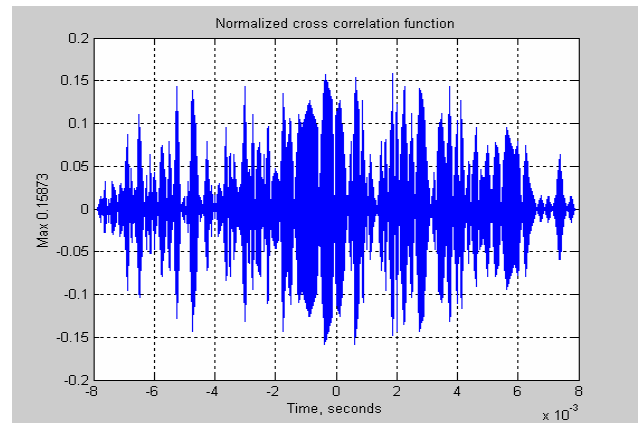
Fig.5. Normalized cross correlation function between the two optimized Short Kasami sequences, the length of sequences is 63 elements
