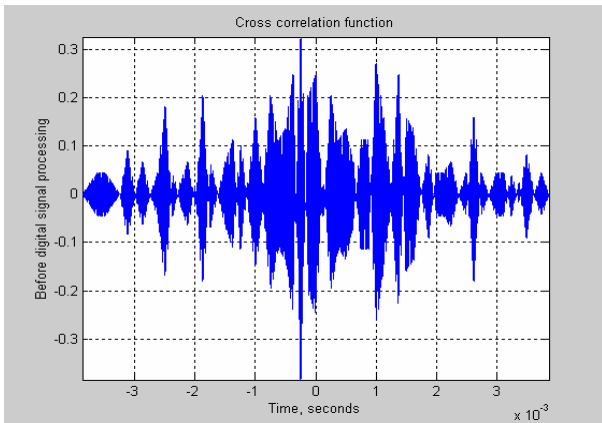
Fig.14. Normalized cross correlation function between the mixture of 10 PN- signals and the reference signal before digital signal processing
