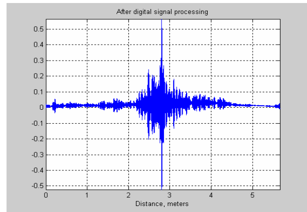
Fig.19. Normalized cross correlation function between the mixture of PN- signals and the reference signal after digital signal processing
