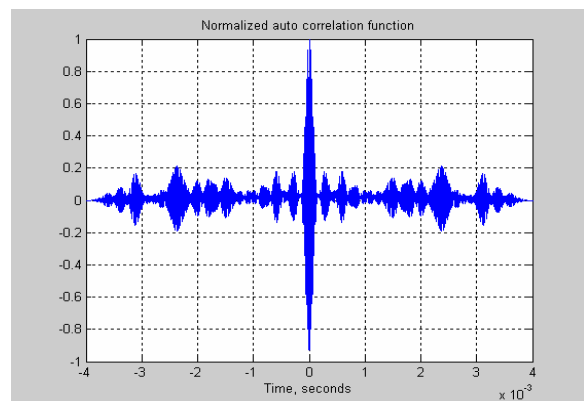
Fig.17. Normalized auto correlation function of the reference signal
