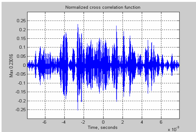
Fig.4. Normalized cross correlation function between the two non optimized Short Kasami sequences, the length of sequences is 63 elements
