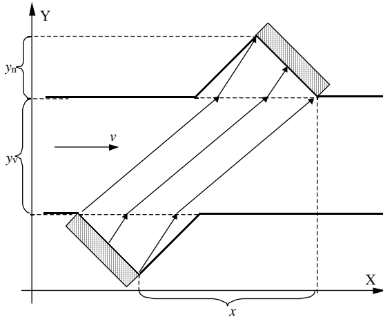
Fig.2. Propagation of an acoustic signal in the measuring channel
