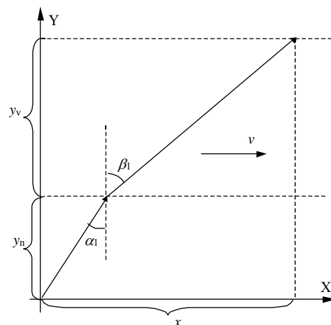
Fig.3. The equivalent diagram of propagation of acoustical signal in the measuring channel
