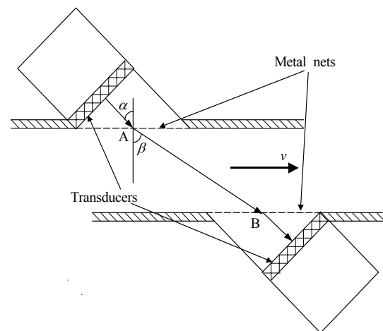
Fig.1. An electroacoustical measurement channel
