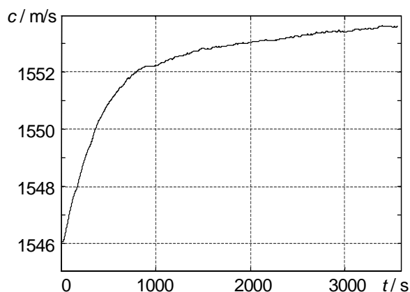
Fig.3. Course of acrylamide polymerisation initiated by potassium peroxodisulphate
