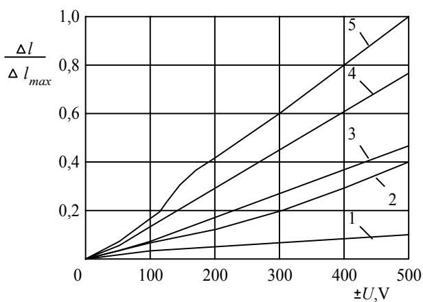
Fig.6 Dependence of piezostack displacement on the supply voltage using different ceramics: 1- ПКП16; 2 - ПКП22; 3 - ЦТС19; 4 - ПКП12; 5 - ПКП7М
